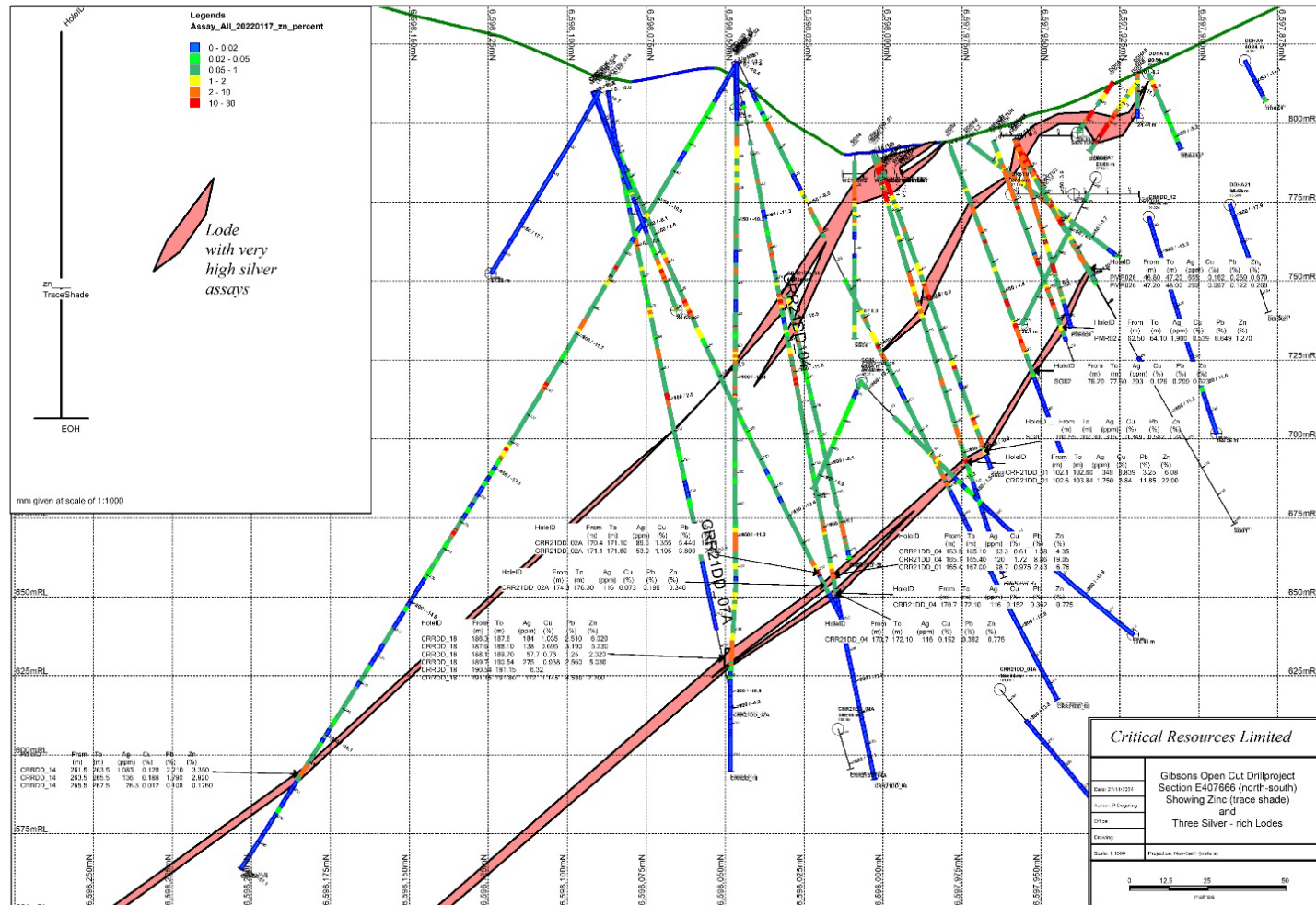
Figure 2: Cross section illustrating the occurrence and distribution three silver-rich lodes (>100ppm silver) within the Gibsons Open Cut deposit.
