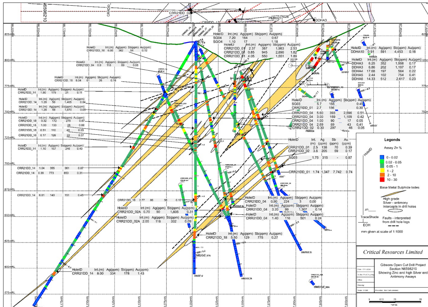
Figure 1: Cross section illustrating the occurrence and distribution of high silver values in the Gibsons Open Cut deposit. High (>100ppm silver) grade silver zones are identified by silver coloured ellipses within the brown stacked massive sulphide lodes (Zn-Pb-Zn).
