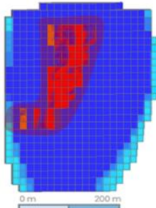
Figure 1: Trieste Lithium Project: Dyke #05 & Dyke #08 along META 3 Trend from Mobile MTm 3D model with superimposed 3D Lineaments.
