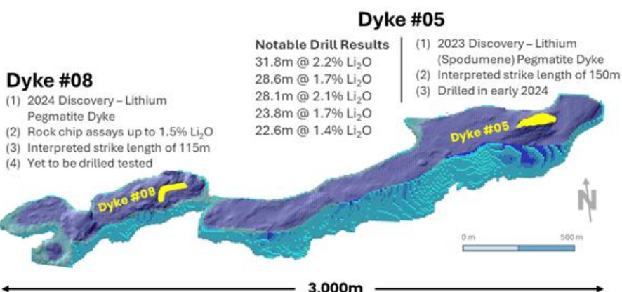
Figure 2: Trieste Lithium Project – Mobile MTm 3D model illustrating the three-metasediment hosted resistive trends.
