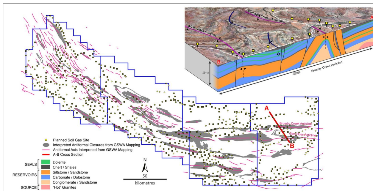
Figure 3: Edmund-Collier Project - Note the numerous large scale antiformal closures that were mapped by the GSWA (Cross Section Interpretation sourced from 1: 100 000 GSWA Tanagdee Geological Series Map) - mapping Information sourced from open file datasets and public reports.
