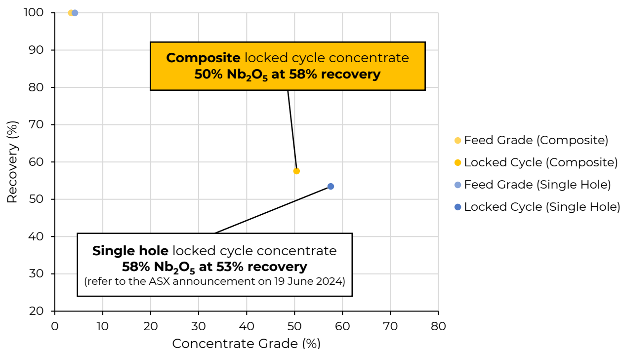
Figure 3: Grade recovery chart of the locked cycle (beneficiation step) tests
