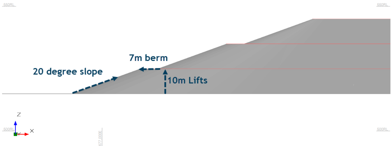
Figure 34 – Waste rock landform design.
