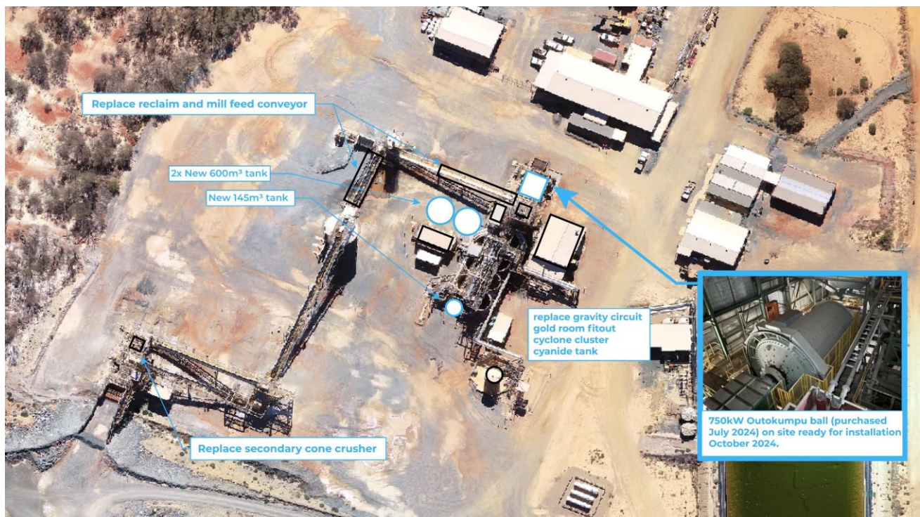
Figure 38 – Andy Well CIL process plant layout.
