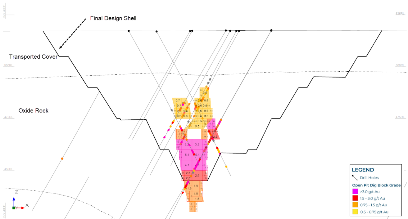
Figure 27 – Cross section at St Anne's South Pit showing dig blocks and stage 1 pit limits, 7082990N.
