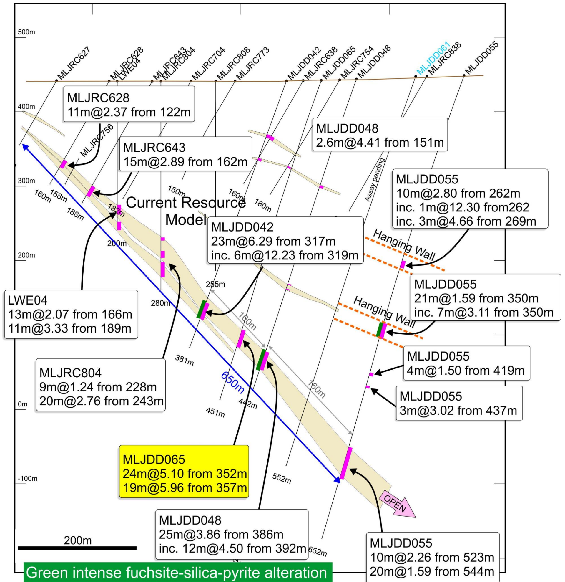
Figure 3. Cross section for LJV4 northern area showing high-grade dipping gold zone containing resource model outline and MLJDD042, 48, 55, 65 being part of a large 650m down dip footwall down dip extension of 160m from MLJDD048. MLJDD061 is waiting for assay and being planned to be drilled respectively.
