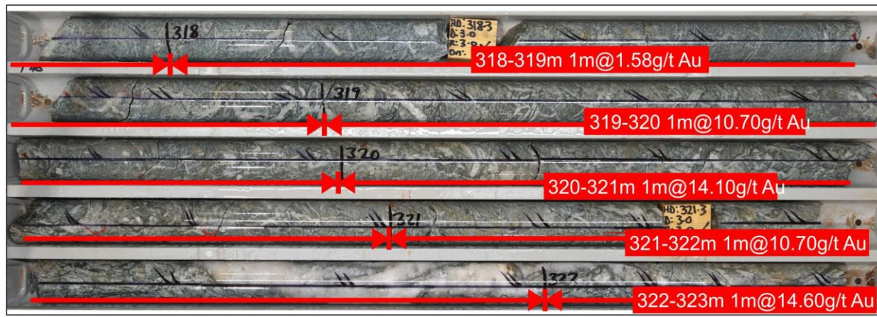
MLJDD042 Silicified ultramafic with fuchsite Alteration
