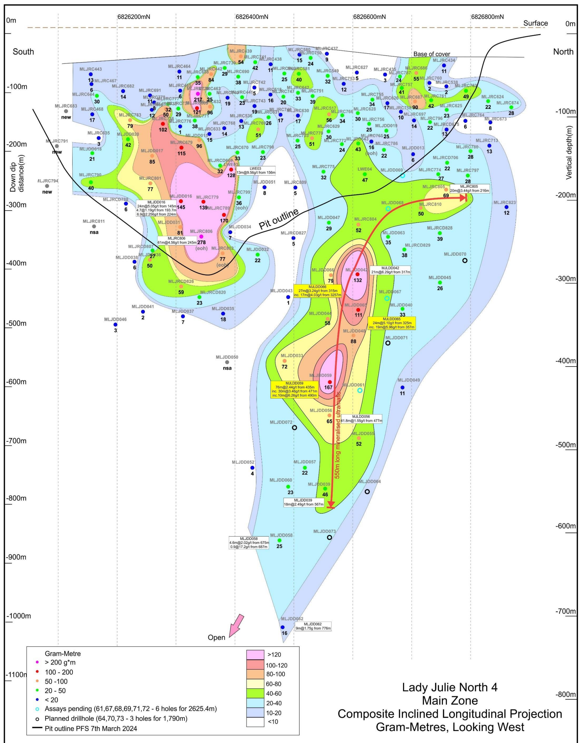
Figure 1. Composite Inclined Longitudinal Projection of LNJ4 in gram-metres. Highlighting continuous mineralisation over the whole 750m strike length, being open at depth in the northern altered ultramafic zone and showing a 550m long SE plunging core zone. New drilled holes awaiting assays (in blue) and further planned holes (in black). New drill results in yellow label and older results in white.
