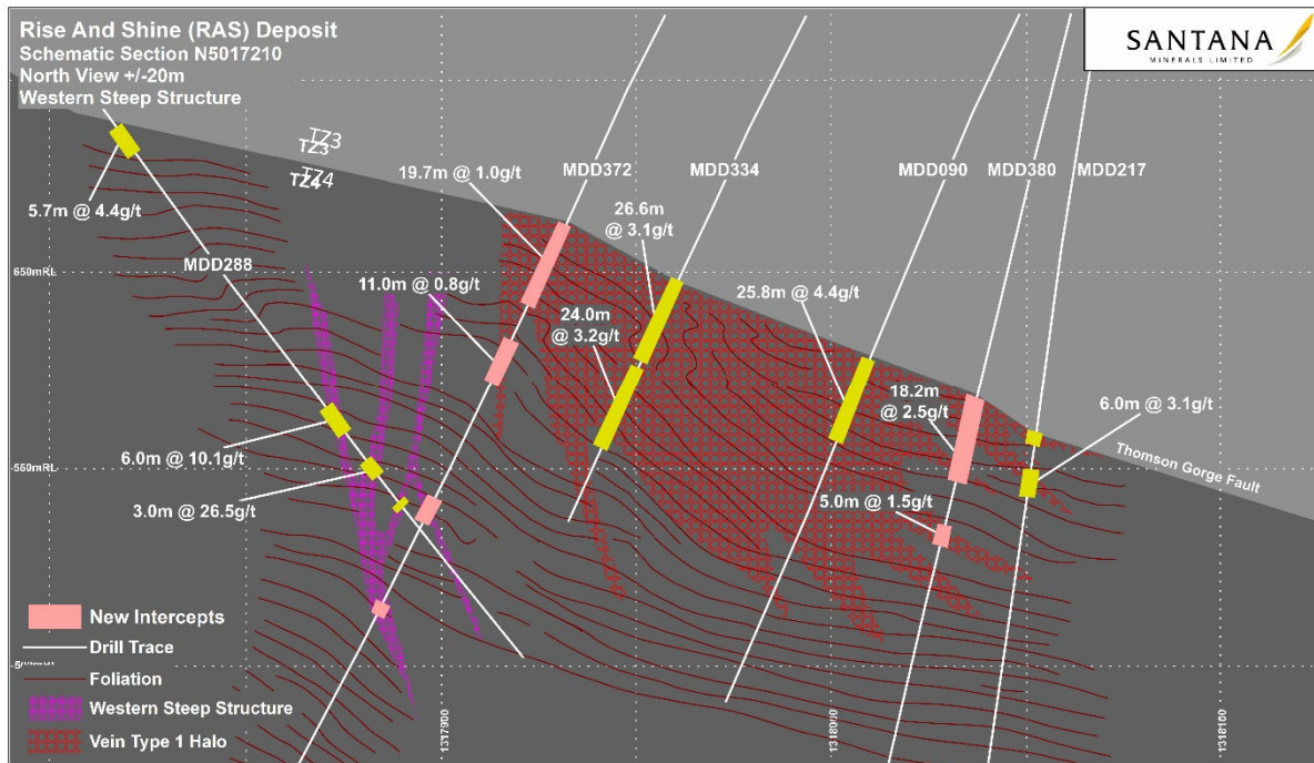
Figure 3. MDD372 section and the correlation with the Western Steep Structure and MDD380 drilled to define eastern extent of RAS orebody for open pit design.
