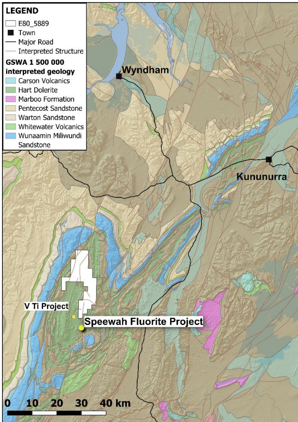
Figure 1: Location plan E80/5889, Speewah, Kimberley region.
