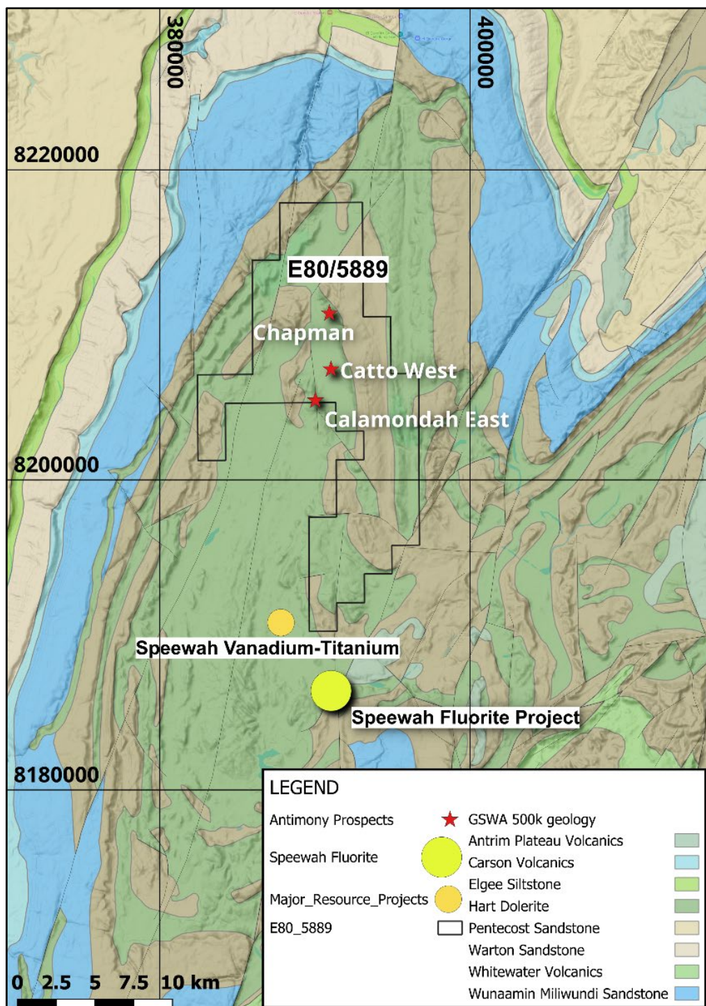
Figure 2: E80/5889 Speewah Project historic antimony anomalies.
