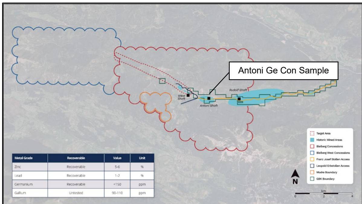
Figure 2: Battery Age exploration tenure, historic mining corridor and production shafts, including Antoni shaft where sample was collected (X474158.8; Y 5165543.6). Inset table demonstrates historical data for the Bleiberg Mine from previous workings 1 .
