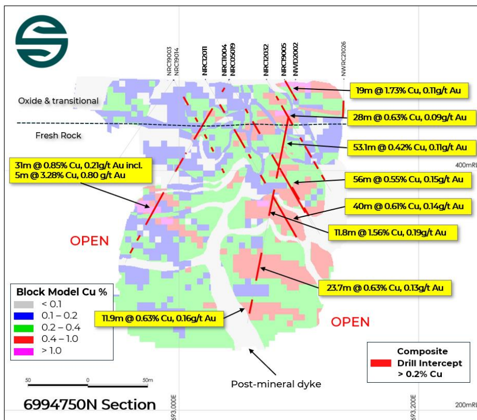
Figure 7. Nanadie Project cross-section 6994750N showing the 2022 MRE block model and all drill traces along with selected copper-gold intercepts.
