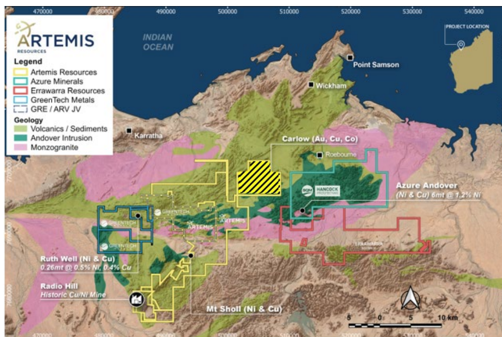
Figure 2. Artemis tenements in Pilbara region of Western Australia with Carlow Tenement hatched
