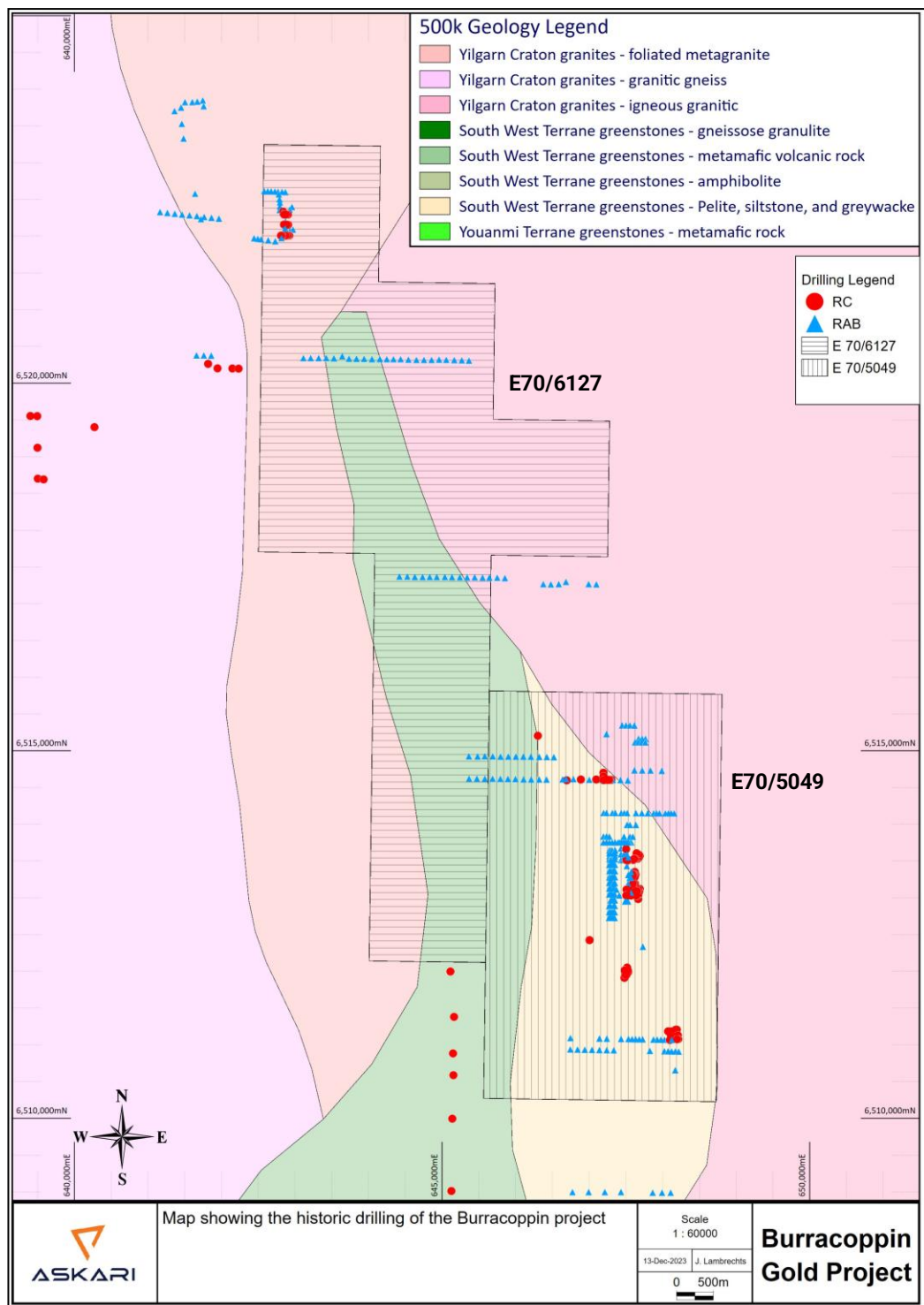
Figure 11: Historic RAB and RC drilling completed on the Burracoppin project
