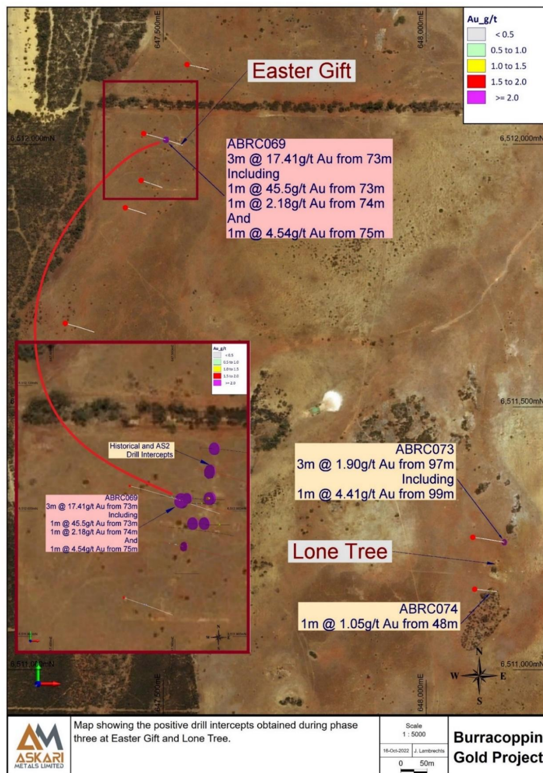
Figure 12: Map showing the drilling reported in Phase III RC drilling program around Easter Gift and Lone Tree
