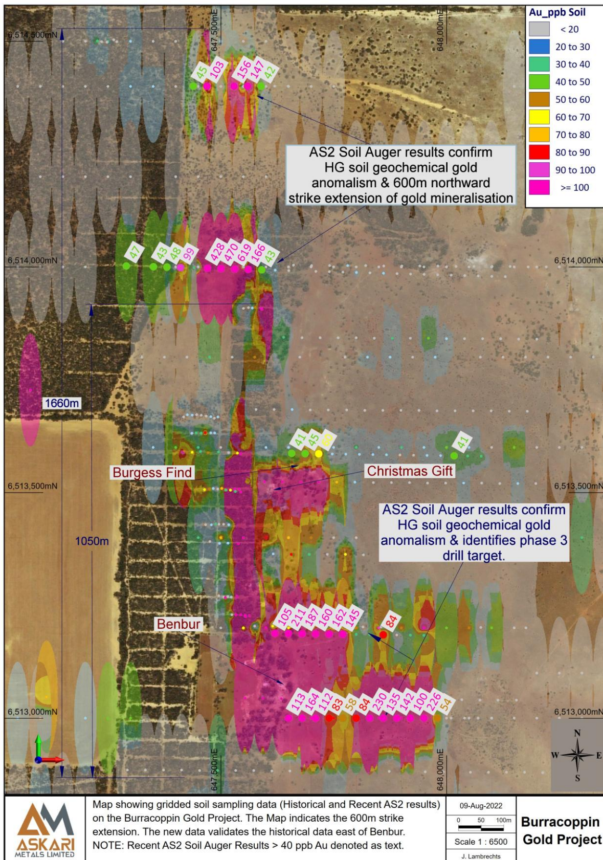
Figure 14: Map of AS2 soil auger results
