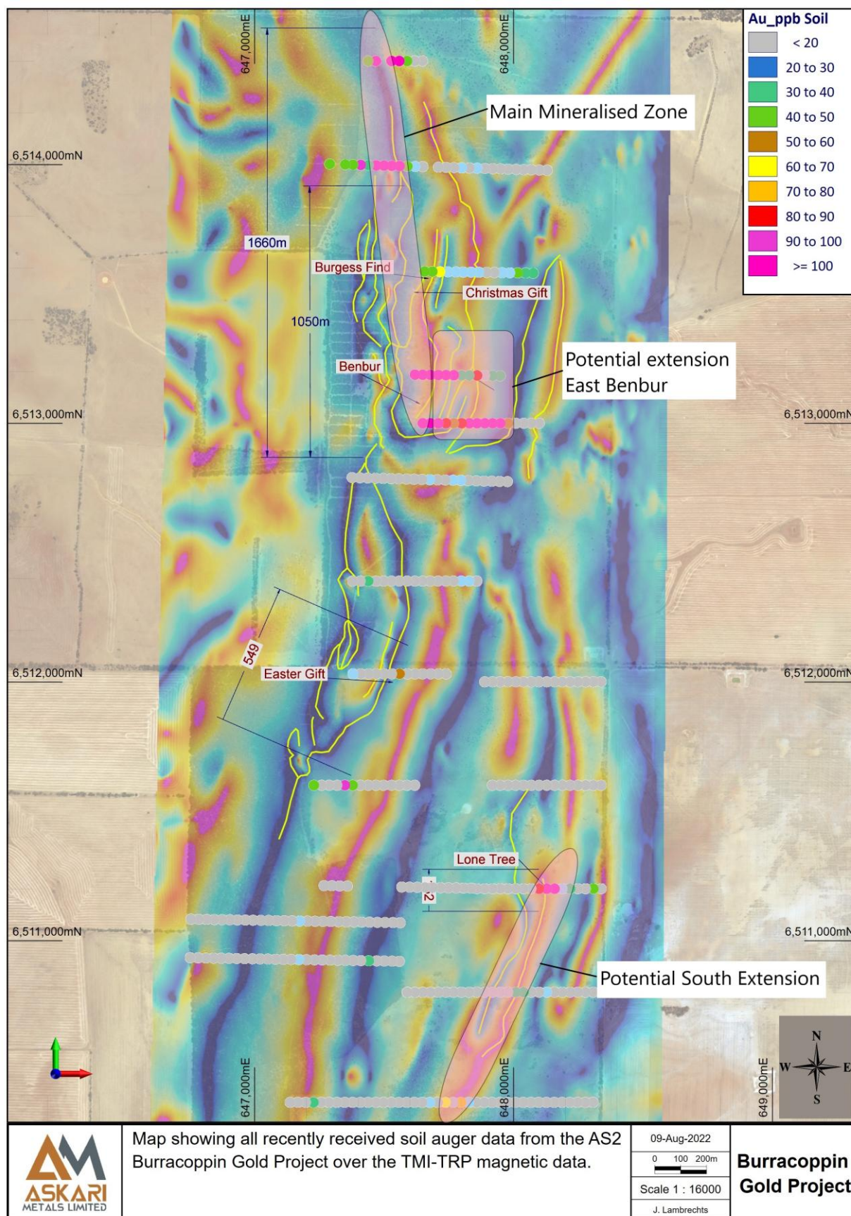
Figure 13: Map of the HD magnetics and AS2 soil auger results
