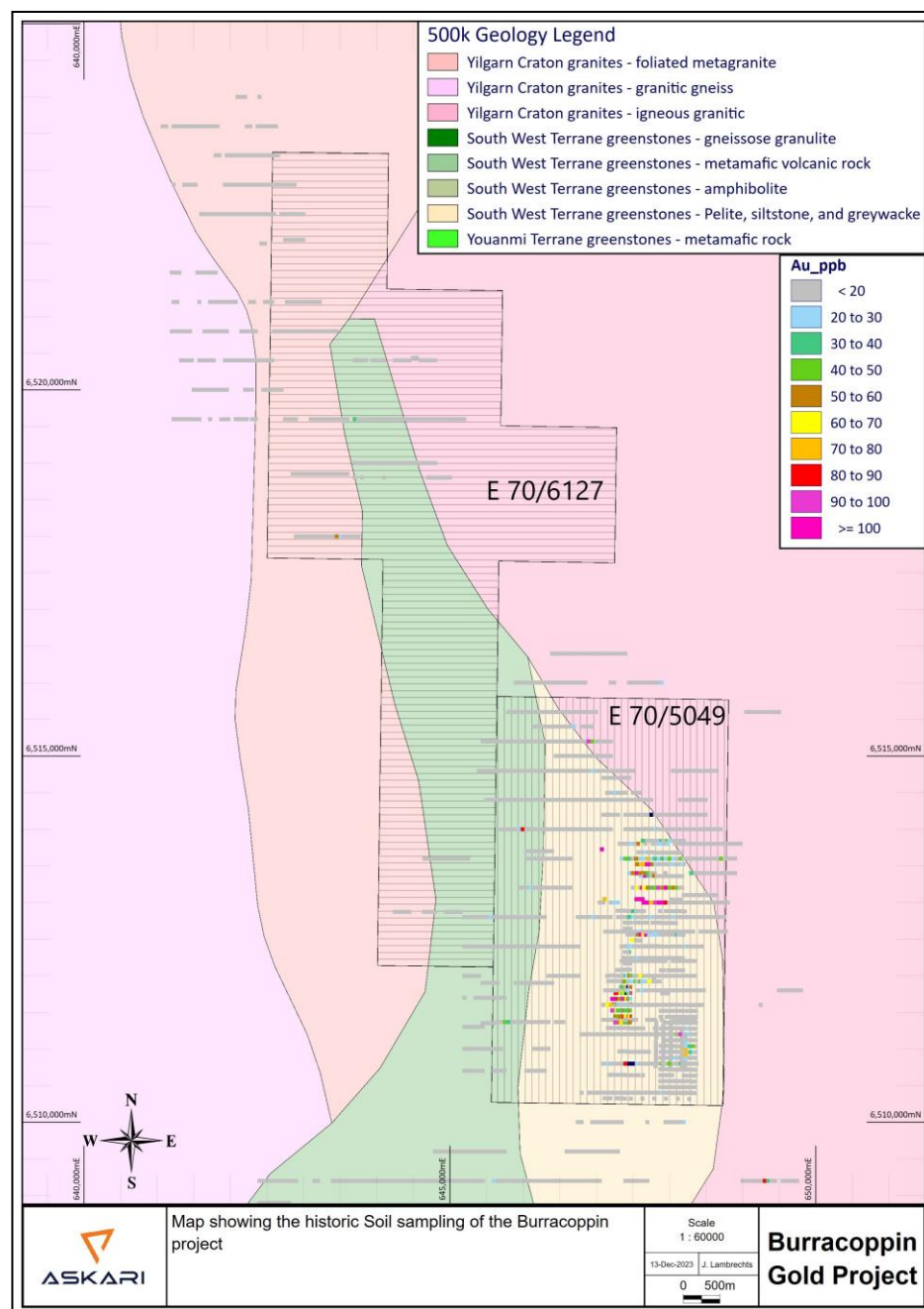
Figure 10: Historic soil sampling completed on the Burracoppin project
