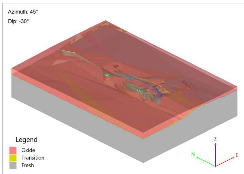
Figure 15: Three-dimensional Diagram of Geological Model of the Benbur-Christmas Gift
