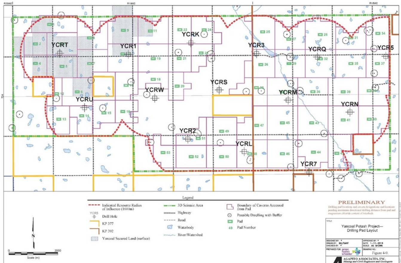
Figure 2-13: Life of Mine Drill Pad Layout
