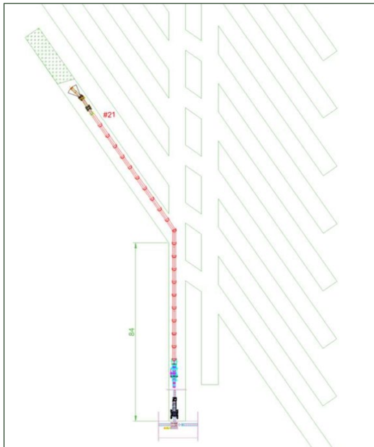
Figure 3-18: Link and Slinger System in Mined-out Room
