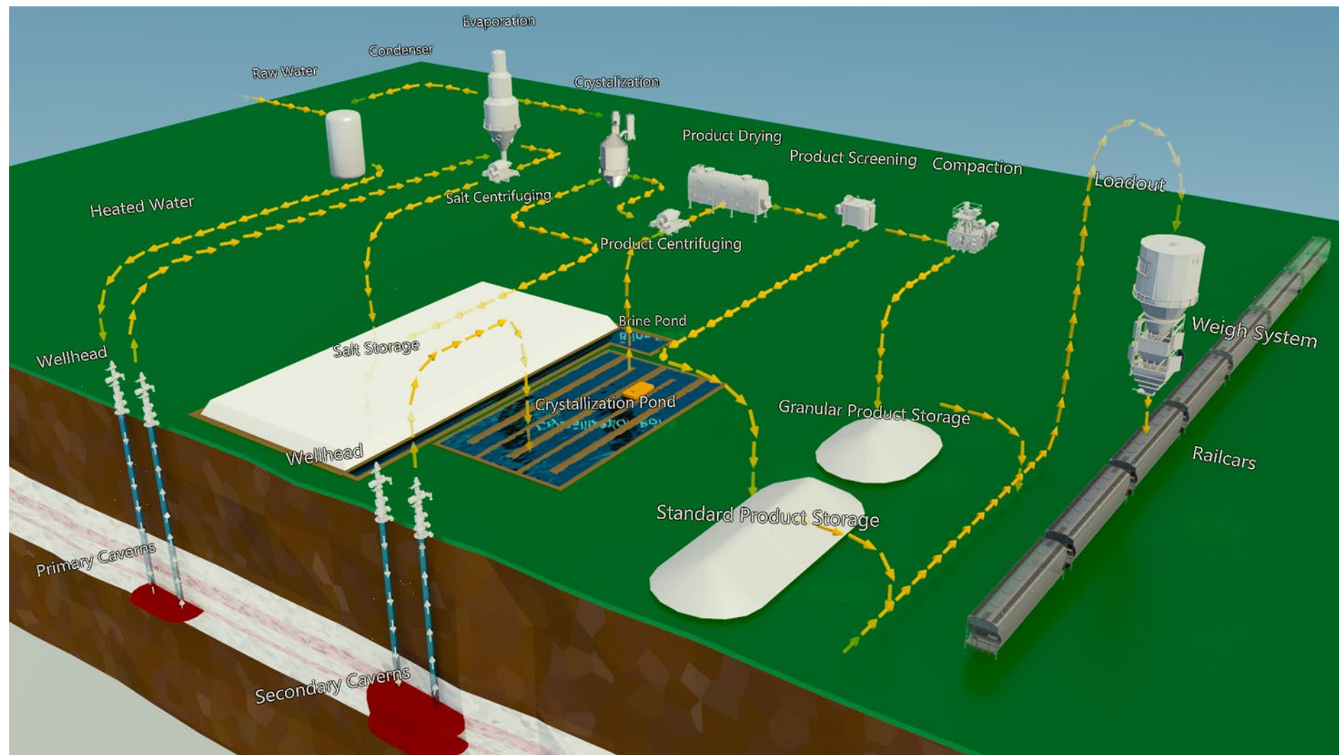
Figure 2-16: Overview of the Primary and Secondary Processing Plants
