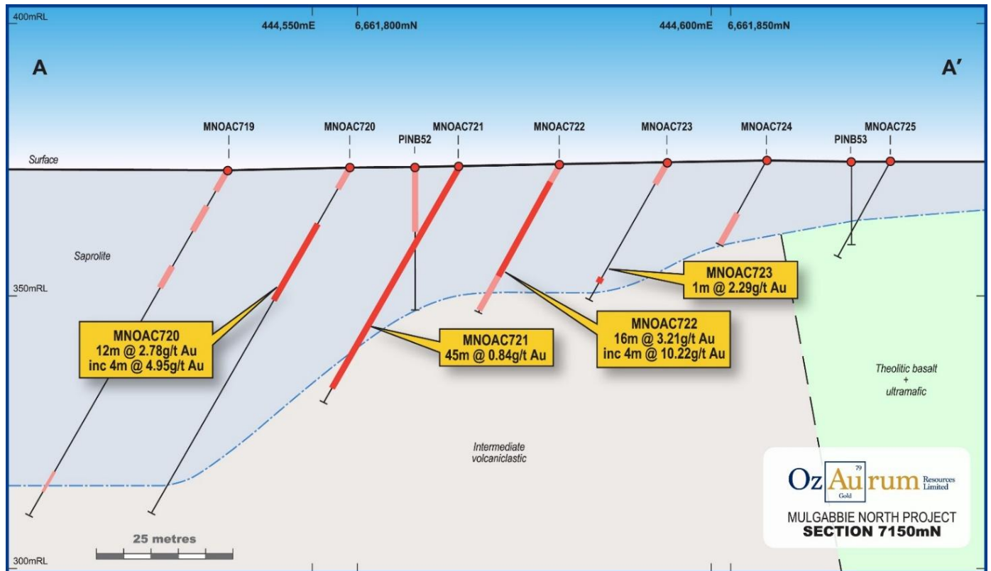
Figure 3: AC drill cross section 7150N
