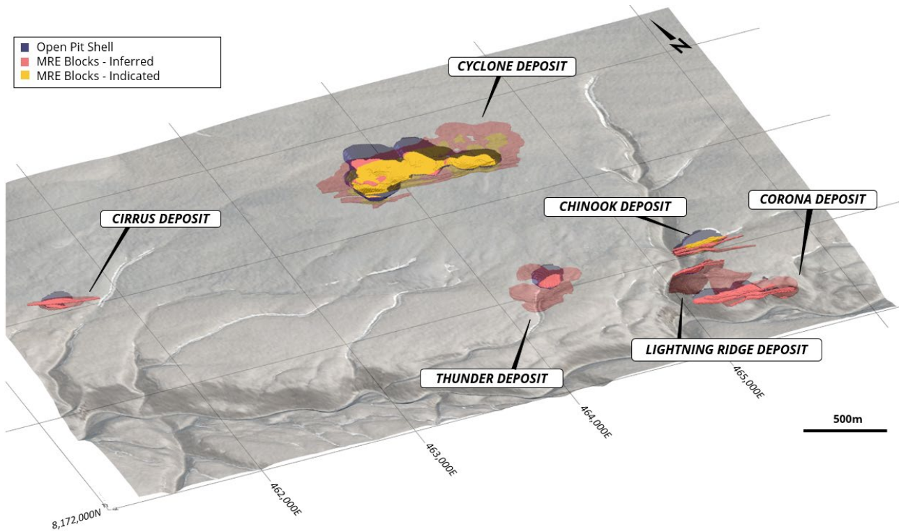
Figure 9: Storm Copper Project open-pit shells and MRE blocks (Indicated and Inferred Classification).
