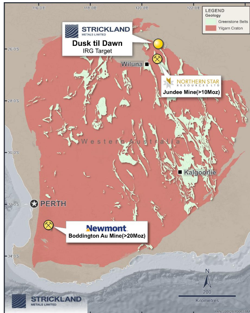
Figure 7: Dusk 'til Dawn Gold Camp in relation to the >20Moz Boddington Gold Mine, both on the margins of the Yilgarn Craton.
