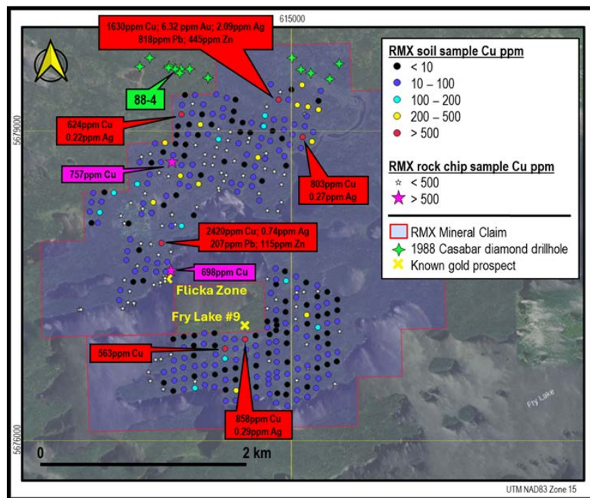
Figure 7: RMX soil and rock chip Cu results for the Flicka Lake project. Elevated and anomalous values are shown for samples containing >500ppm Cu. The locations of the Casabar Resources 1988 diamond drill hole collars are also shown.
