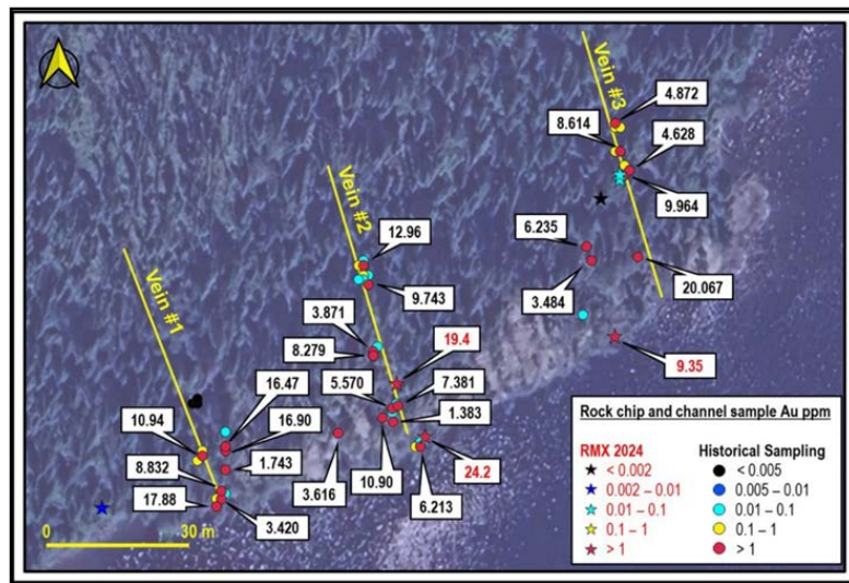
Figure 5: RMX rock chip and Troon Ventures historical rock chip and channel gold results for the Flicka Zone. Values of > 1ppm (1 g/t Au) are shown. The location of three mineralised quartz veins as mapped by Troon Ventures are also shown. Note that the mapped location of these veins and of some historical samples may have a GPS error of up to 10m – most significantly, the 9.35ppm (9.35 g/t Au) RMX sample is interpreted to be from Vein #3.
