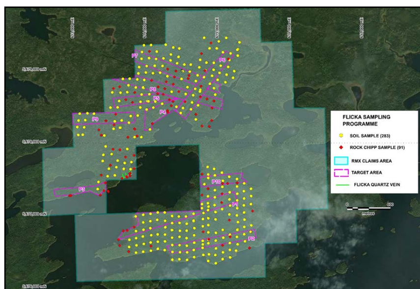
Figure 3: Rock Chip and Soil Sampling Coverage over target Areas
