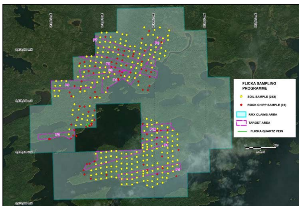
Figure 2: Sampling targets based on geological, structural, geophysical and historical sampling data.
