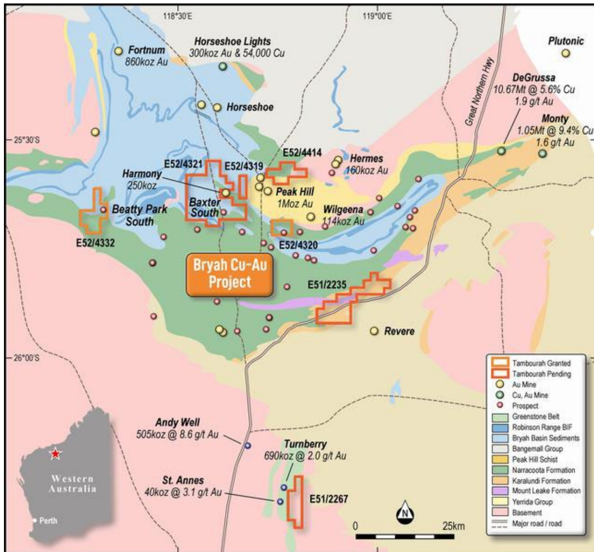
Figure 9: Bryah tenement locations on geology, showing gold and copper-gold deposits
