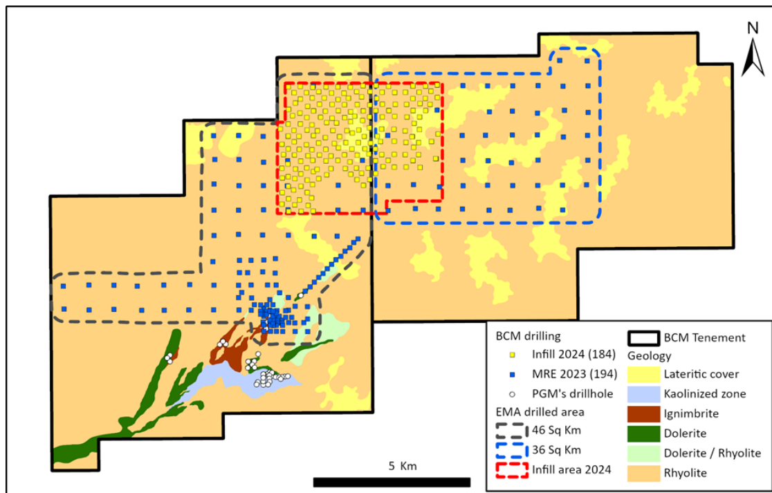
Figure 1 - Ema REE project – Mineral Resource covering 82 km 2 with auger holes on 800m spacing and infill auger holes on 400m centres over 20 sq km.
