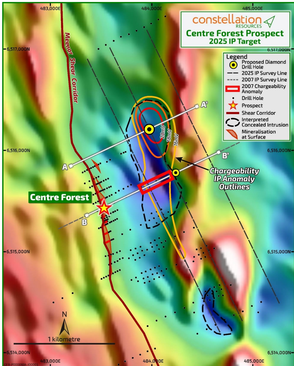
Figure 2: Centre Forest Prospect showing surface projection of mineralisation over a 1.1km strike draping the TMI aeromagnetic image, interpreted concealed intrusion and modelled DDIP chargeability outlines.
