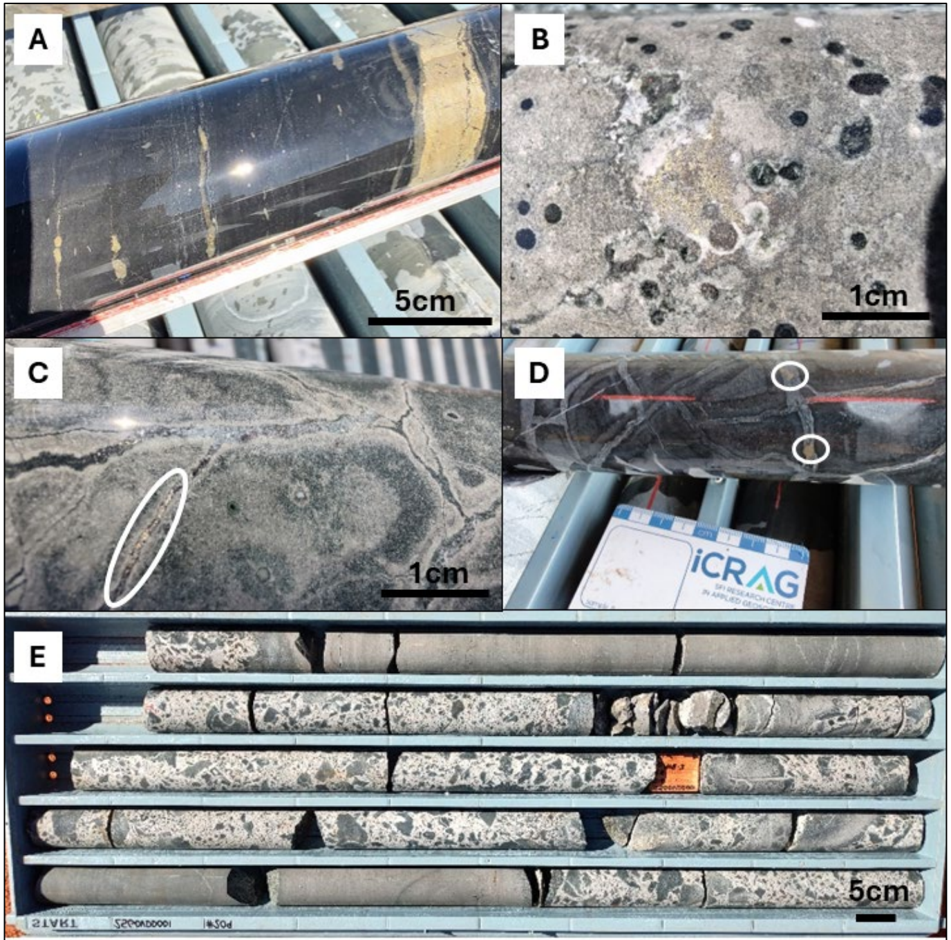
Figure 4: (A) lenses of banded pyrite within interbedded shale-volcaniclastic rocks, considered responsible for the conductive response (835m); (B) Chalcopyrite (mineralogy confirmed with XRF) with pyrite and quartz-carbonate veining and within the basalt sequence (1,031m); (C) Chalcopyrite within pyrite veining (confirmed with XRF), at 1,026m; (D) Chalcopyrite with quartz-carbonate veining, at 878m; (E) Carbonate matrix breccia with basaltic clasts, with pyrite both disseminated and rimming clasts (918m), potential VHMS feeder?
