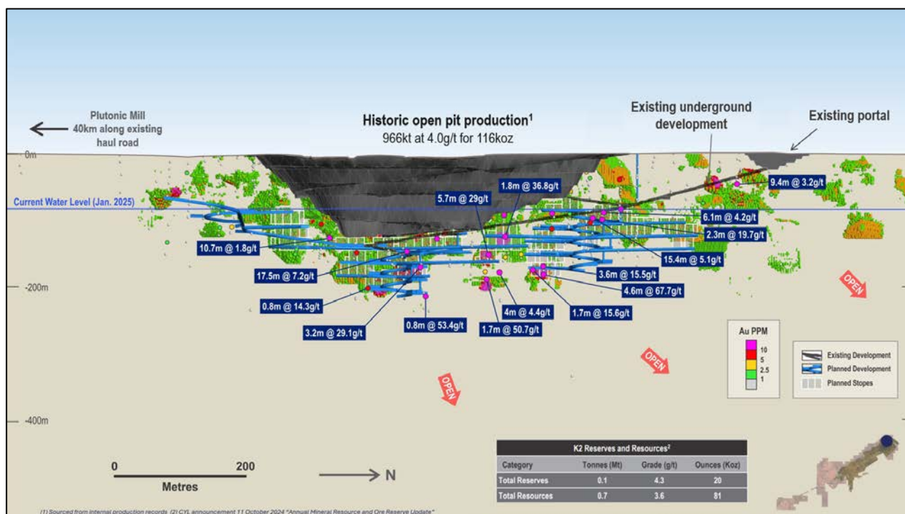
Figure 4: K2 showing existing decline, current water level, planned stopes and exploration potential
