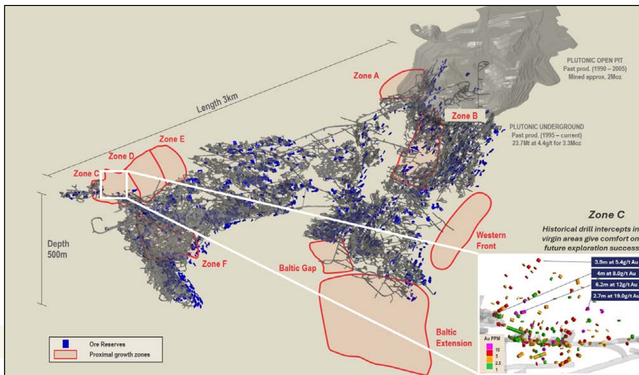
Figure 3: Plutonic Underground with proximal growth zones
