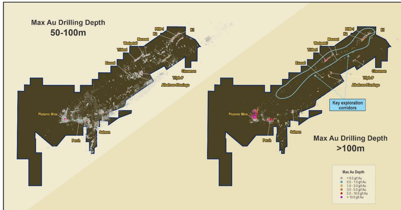
Figure 7: Plutonic gold belt showing mineralisation below 100m versus drilling density below 100m
