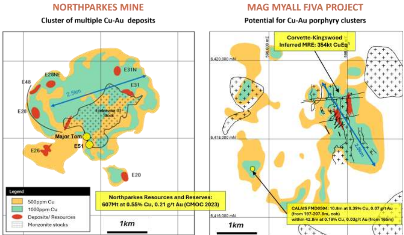
Figure 5. Northparkes porphyry cluster system next to Magmatic’s Kingswood – Corvette area at the same scale.
