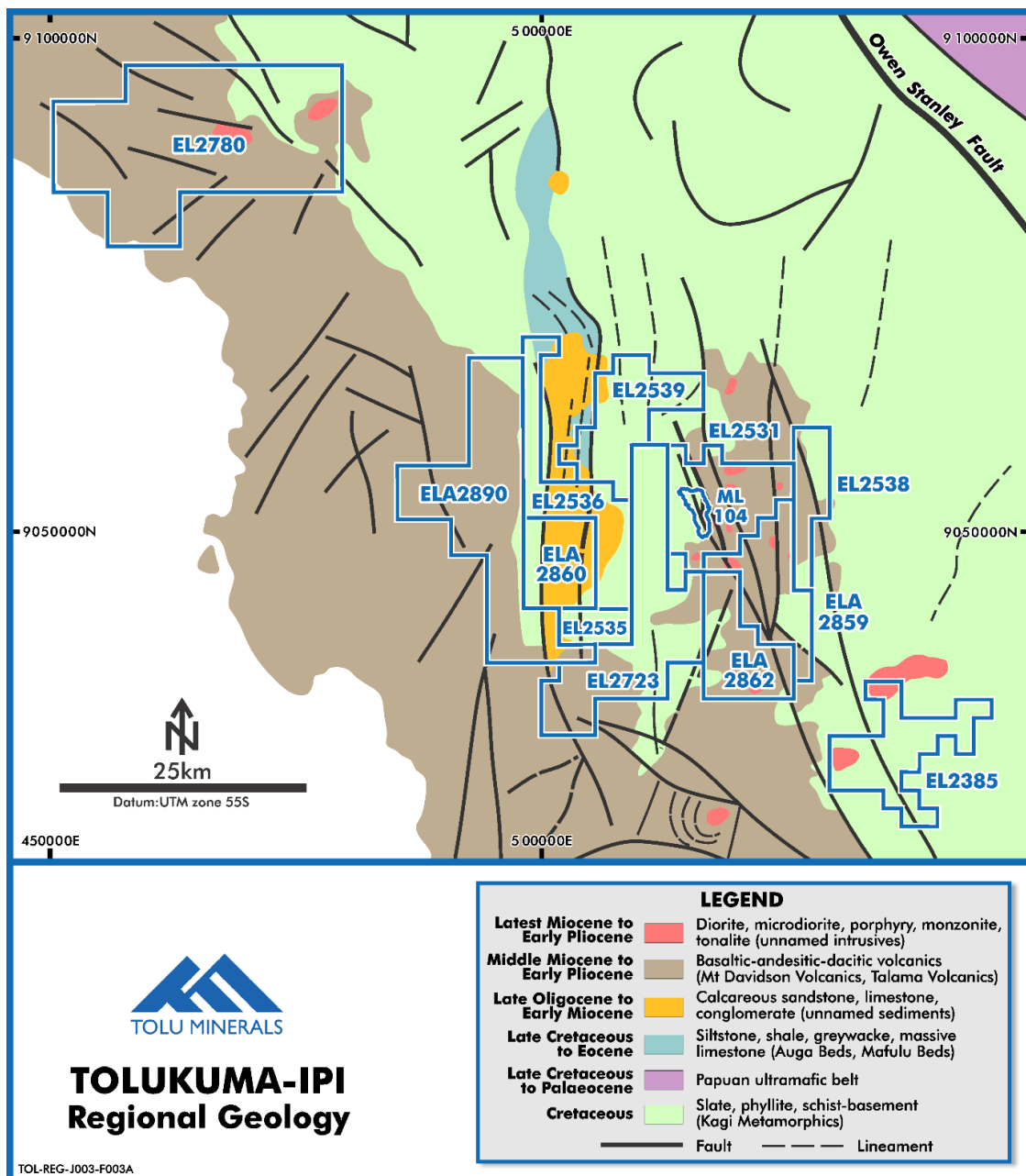
Figure 1: Location and Regional Geology of Ipi River EL2780 and Tolukuma Tenements
