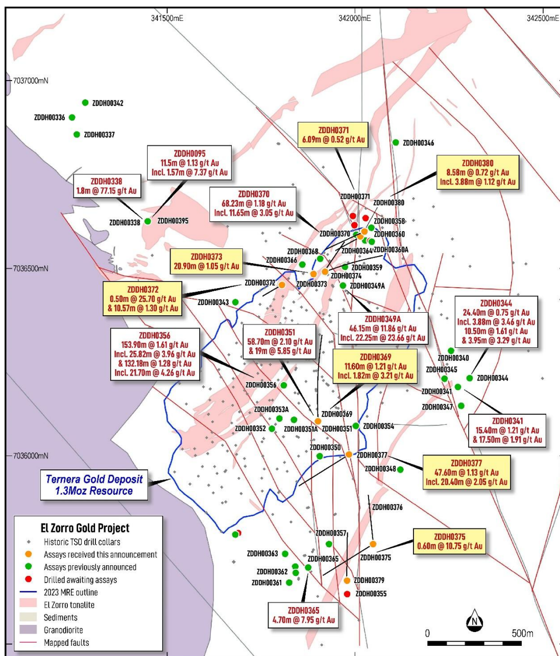
Figure 1: El Zorro Gold Project – Ternerá Area. Drill locations in the current program, with new results highlighted in gold. Previously announced results shown in white (refer ASX Announcements 23 March 2021, 25 June 2021, 3 November 2021, 8 November 2022, 18 September 2023, 13 June 2024, 2 July 2024, 28 October 2024, 16 January 2025 and 20 March 2025). Datum PSAD56 19S.
