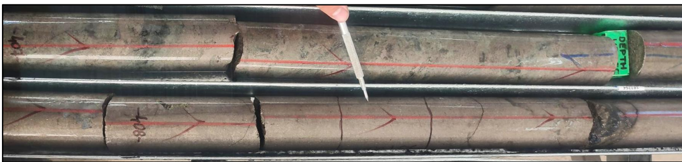
Figure 6. Core photograph from 407.7m to 408.8m in ZRSD25182 showing massive pyrrhotite mineralisation – 9.5g/t Au.
