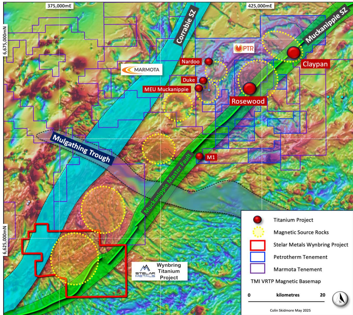
Figure 2: Wynbring tenement ELA2025/0001 in relation to Petratherm's Muckanippie Titanium Project showing key structures and circular magnetic source rocks on magnetic imagery
