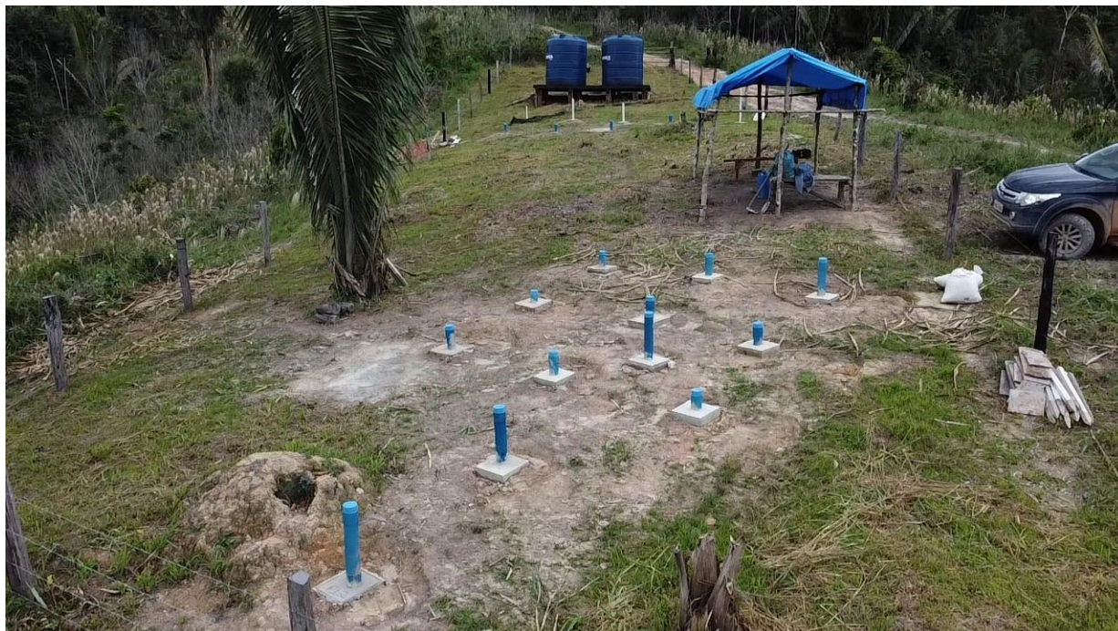
Figure 4. View of the field trial injection and extraction wells, water storage and solution preparation tanks and distribution system where solutions samples were sourced.
