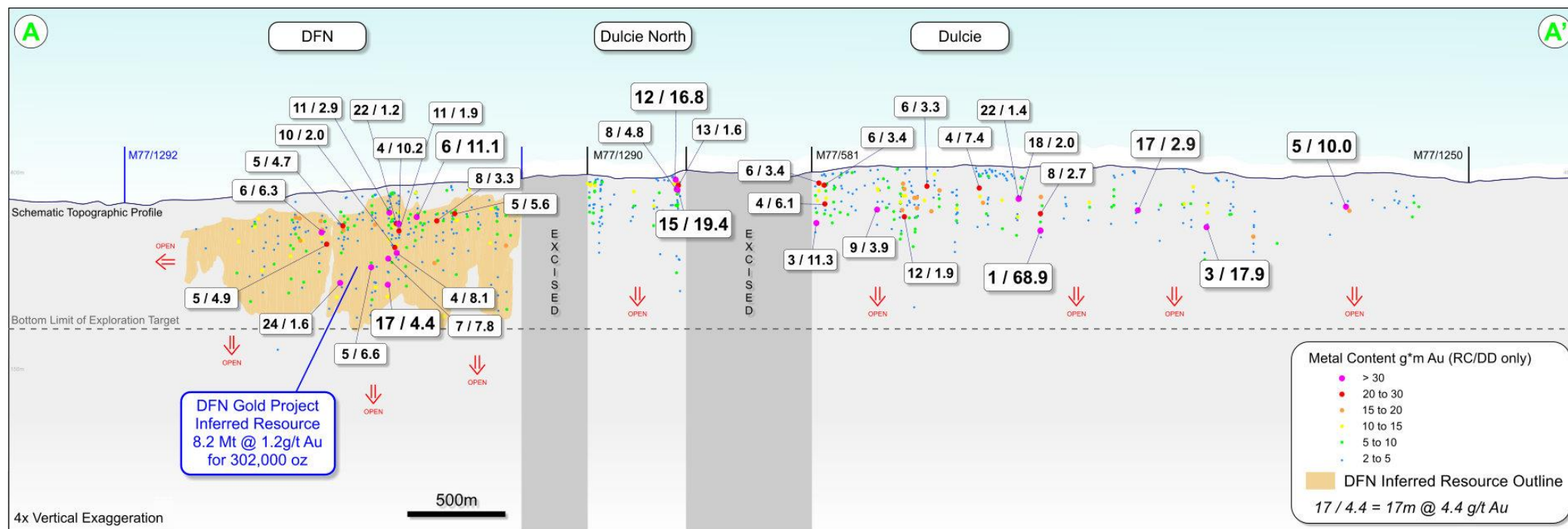
Figure 2: Long-section illustrating the existing DFN Inferred Mineral Resource and exploration drill intercepts, highlighting open-ended mineralisation and potential for extensions (including RC, diamond, aircore and RAB). For detailed drill intercepts, refer to the previously released ASX announcements listed in the Competent Persons Statement section at the end of this release.
