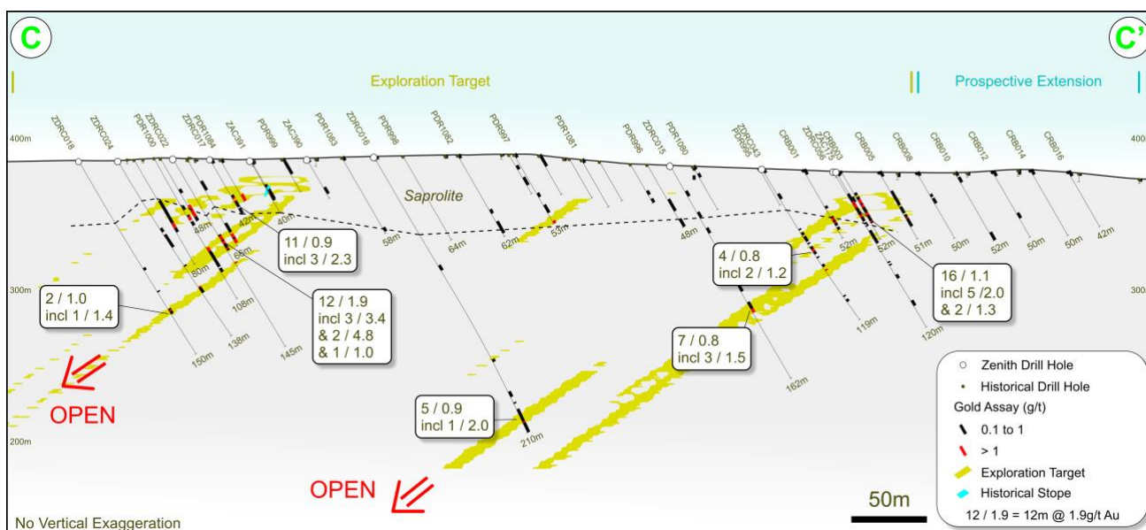
Figure 4: Cross-section C-C' (Dulcie - 'Scott's Grey') illustrating Exploration Target lodes in yellow and prospective open-ended mineralisation.
