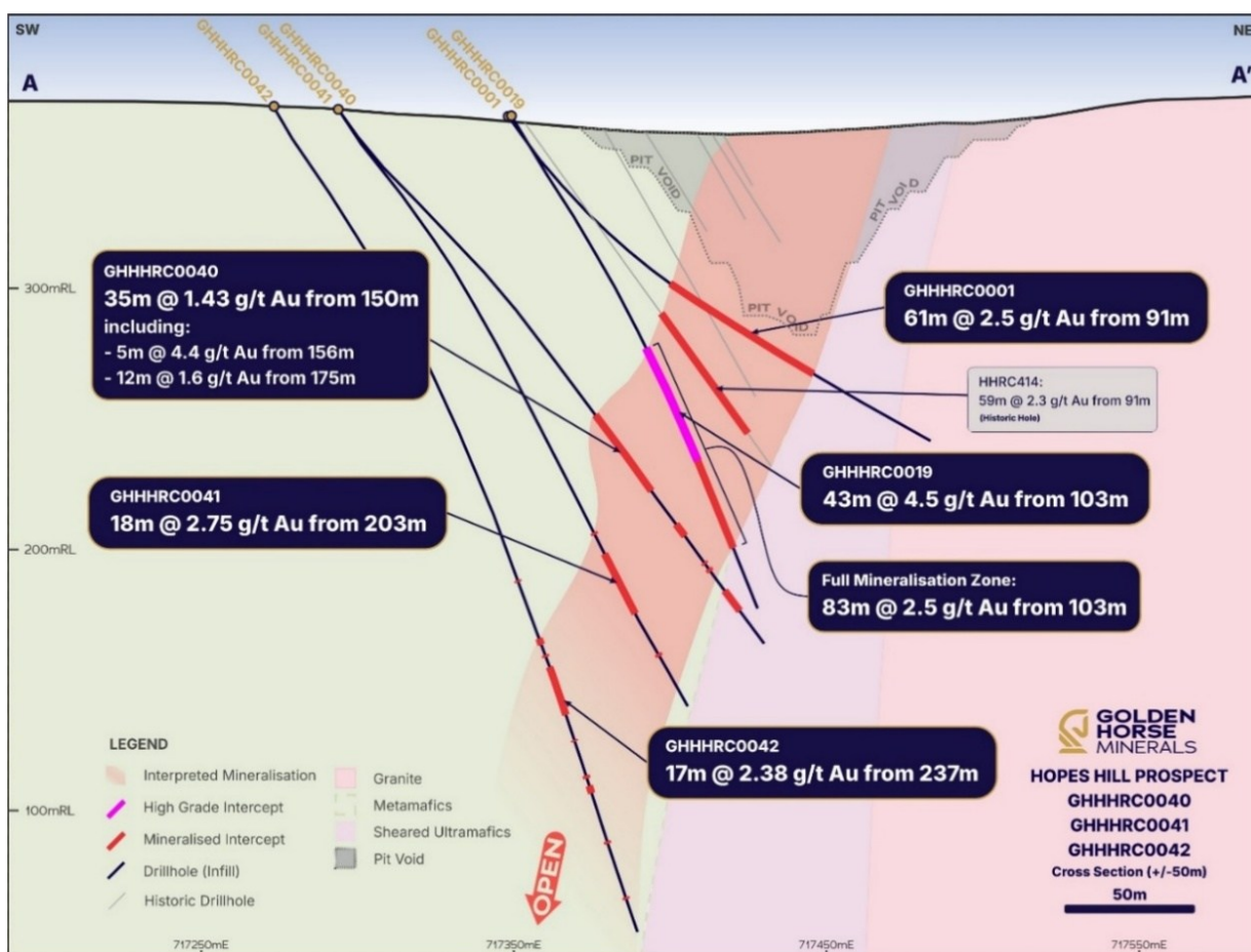
Figure 3: Hopes Hill Cross Section – Significant intercepts received most notably GHHHRC0019, 40, 41 and 42.
