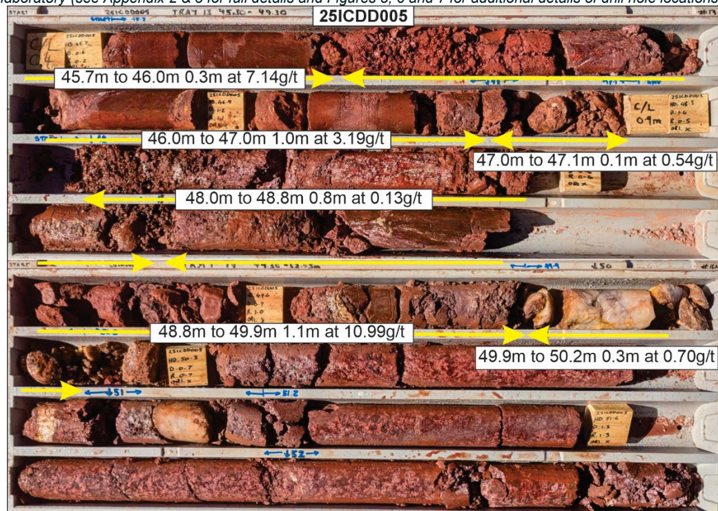
Figure 3 - Drill core from hole 25ICDD005 ( \sim 60 to 083^\circ ), trays 13 and 14 showing sheared and veined gabbro between 45.7m to 50.2m which were assayed and returned a significant intercept of 4.5m at 3.94g/t Au (intervals of core loss are included at 0.0g/t). Photo shows HQ3 (61.1mm diameter) whole-core prior to cutting and sampling. Hole depths & core loss (C/L) are marked on core blocks. Au grades are 50g fire assay as reported by NAGROM laboratory (see Appendix 2 & 3 for full details and Figures 5, 6 and 7 for additional details of drill hole locations).
