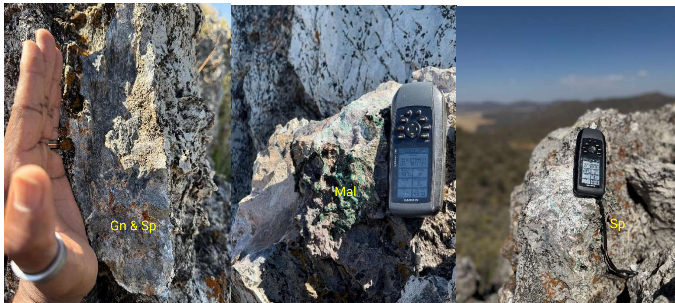
Image 2a: Gossan 2, sphalerite (Sp) galena (Gn) in brecciated doleomite
