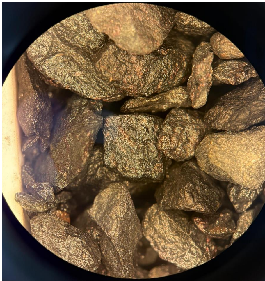
Figure 3 - Example of bornite rich RC drill chips from 80.77 to 91.44m in DAN25012. Cautionary Statement: The Company cautions that, with respect to any visual mineralisation indicators, visual observations and estimates of mineral abundance and uncertain in nature and should not
