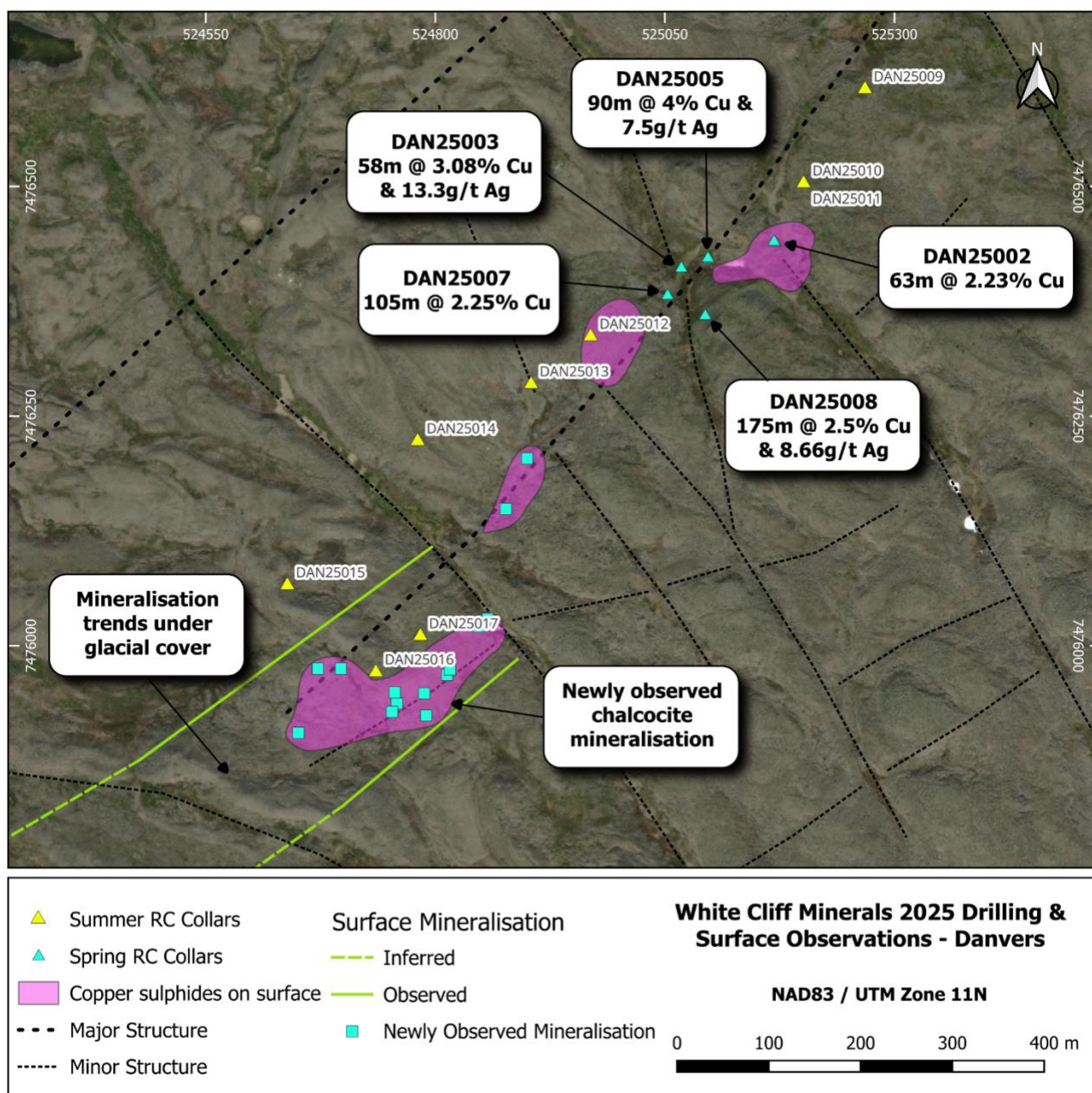
Figure 4 - Map of 2025 Spring and Summer RC drillholes at the Danvers Breccia System.
