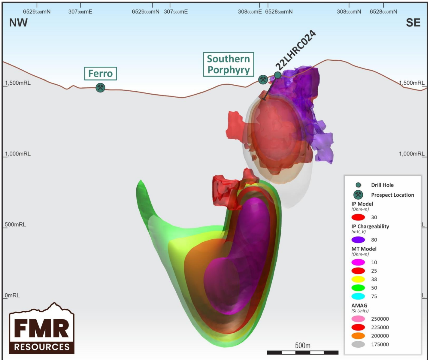
Figure 5. Cross section A-A', looking north-east, showing the spatial arrangement of the geophysical models at Southern Porphyry in relation to the Ferro deposit (SUH) (window +/- 250m).
