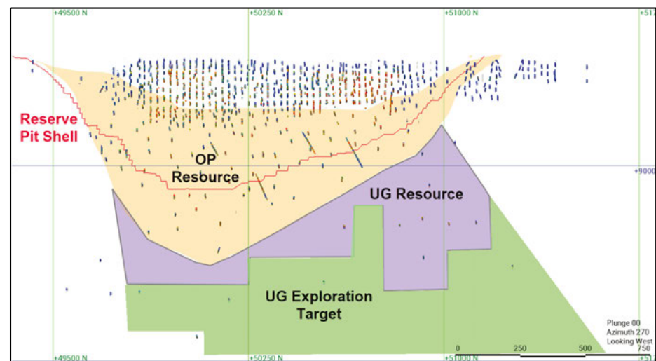
Figure 3.2: Gruyere long section looking west
