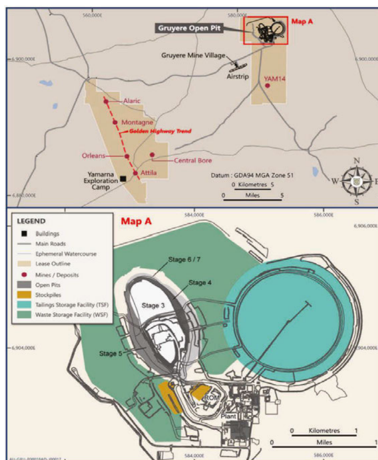
Figure 3.14: Gruyere operating sites and infrastructure
