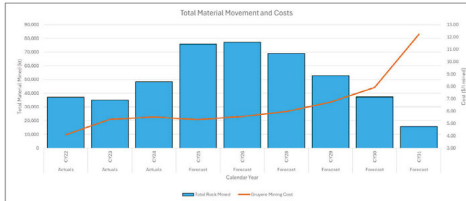
Figure 3.10: Gruyere open pit material movement and costs
