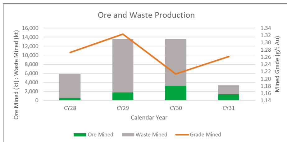
Figure 3.12: Golden highway open pit mining schedule
