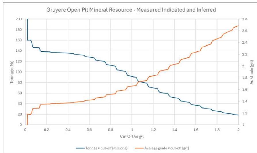
Figure 3.5: Gruyere open pit Mineral Resource grade and tonnage curves
