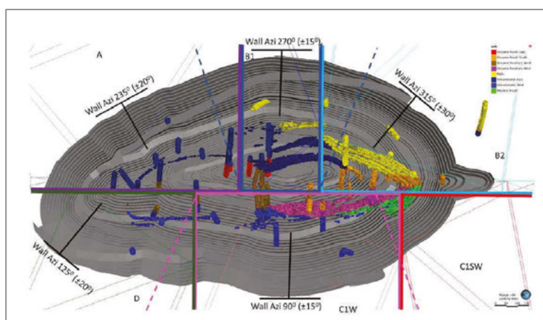
Figure 3.7: Plan view of the various geotechnical design sectors in the Gruyere pit
