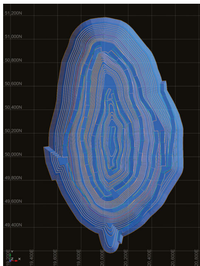
Figure 3.8: Gruyere final pit design, plan view
