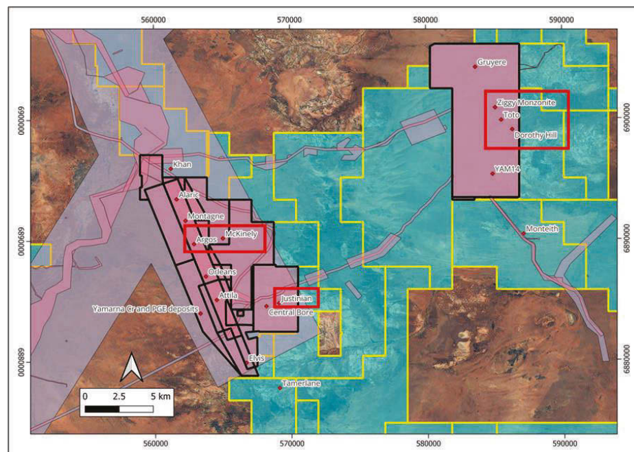
Figure 3.4: Key exploration prospects within the Gruyere JV tenements
