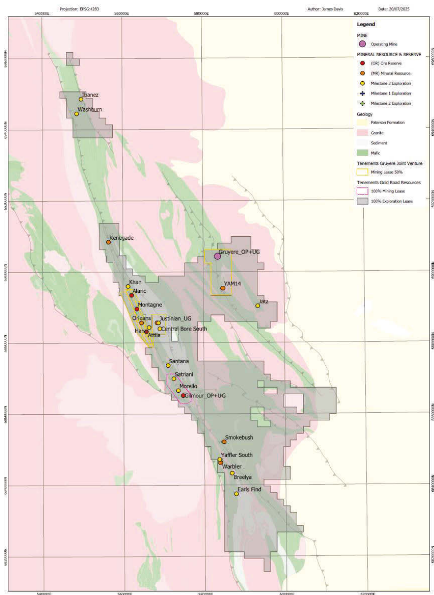
Figure 4.2: Geological setting of the Gilmour and broader Yamarna areas
