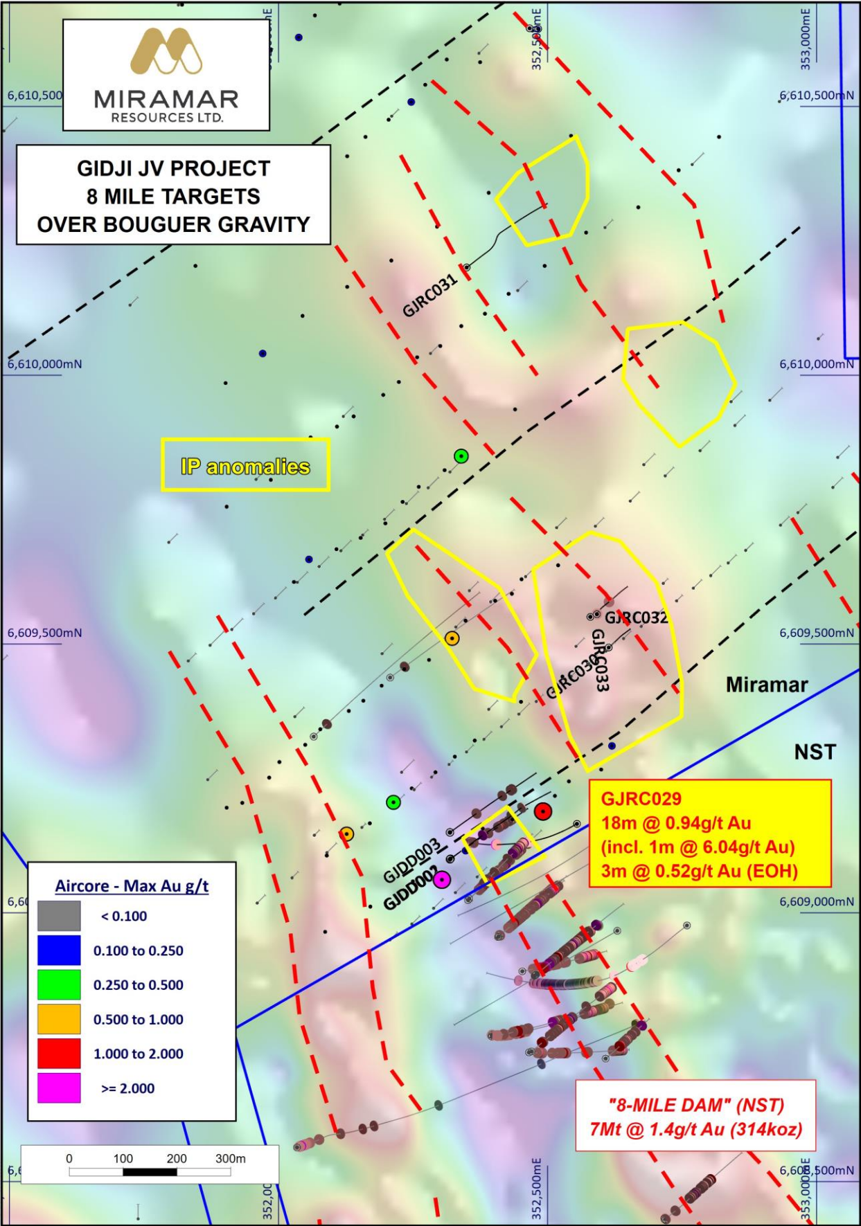
Figure 2. 8 Mile prospect showing drill targets (red dashed lines) over Bouguer gravity image.
