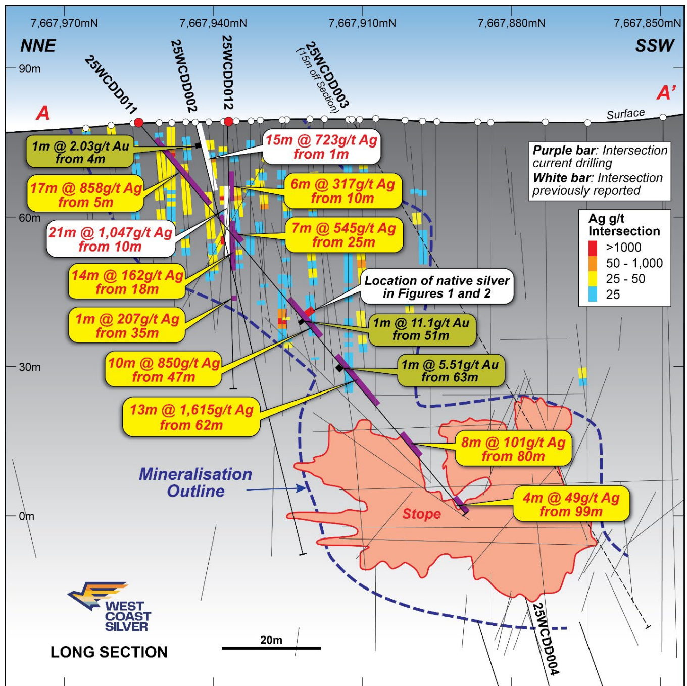
Figure 0—Long section showing drill holes 25WCDD001, 25WCDD002, 25WCDD003, 25WCDD004, 25WCDD011 & 25WCDD012 and previously reported drill holes 25WCDD001, 25WCDD002, 25WCDD003, 25WCDD004, 25WCDD011 & 25WCDD012 (looking ESE, refer to ASX announcement dated 7 th July 2024);
