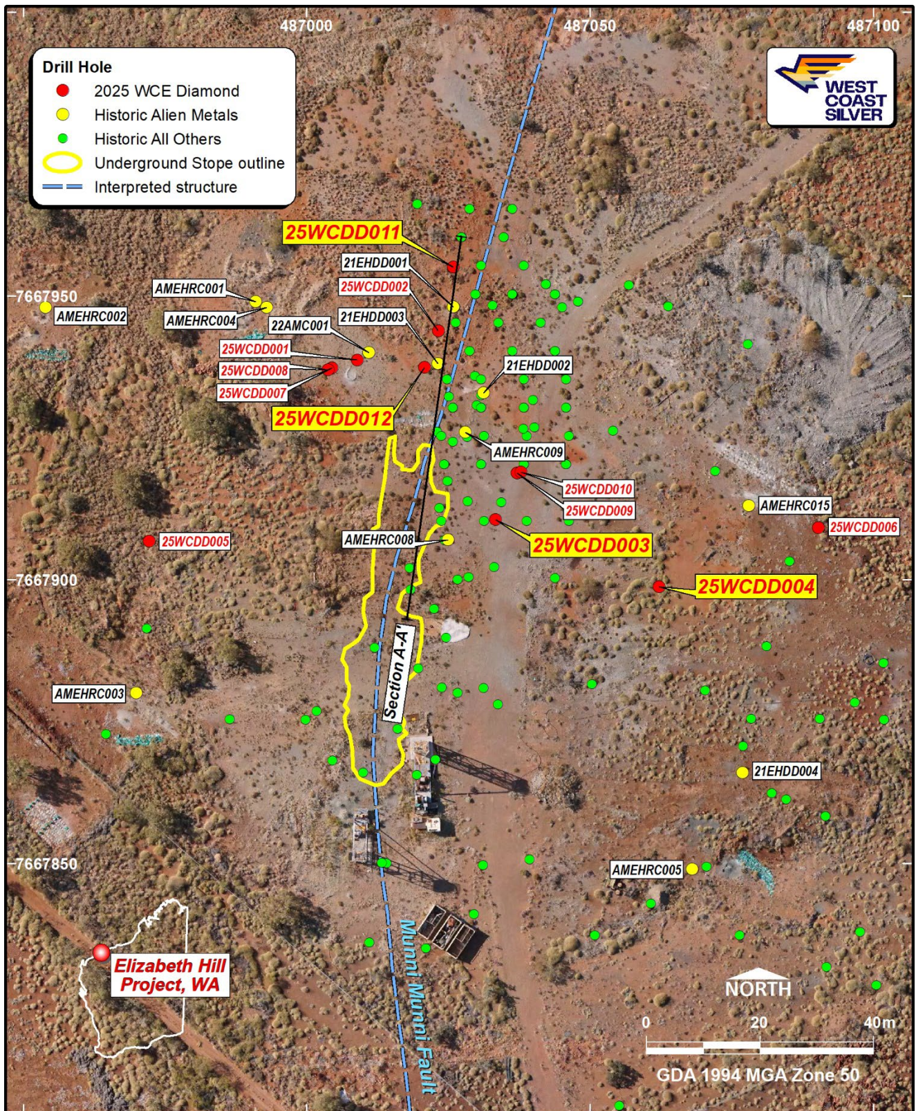
Figure.9- Plan view of 868@West Coast Silver Diamond core drilling and historical drilling
