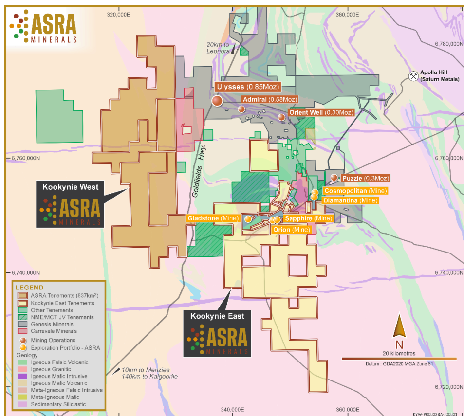
Figure 2 – Leonora South Gold Project
