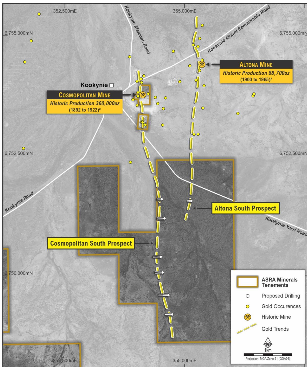
Figure 1 – Completed Drilling at Cosmopolitan and Altona South Prospects
