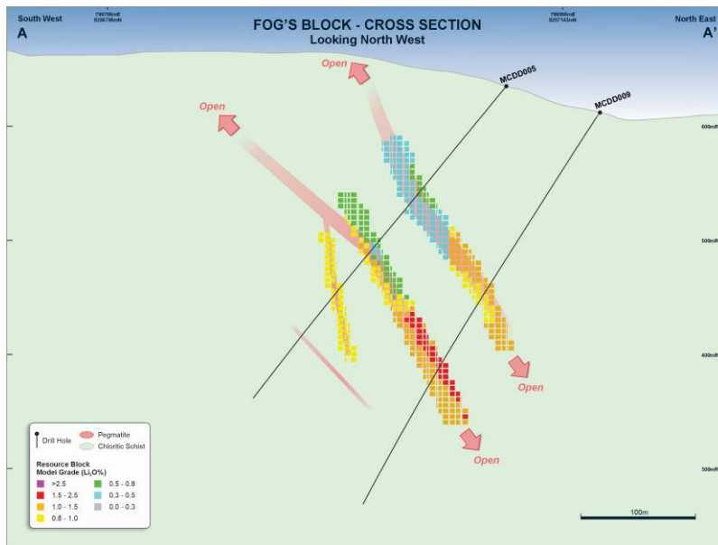
Figure 9 – Fog's Block cross section A-A'.
