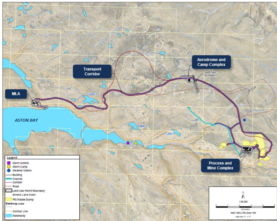
Figure 1: Storm Copper Project PEA infrastructure and facility general layout.
