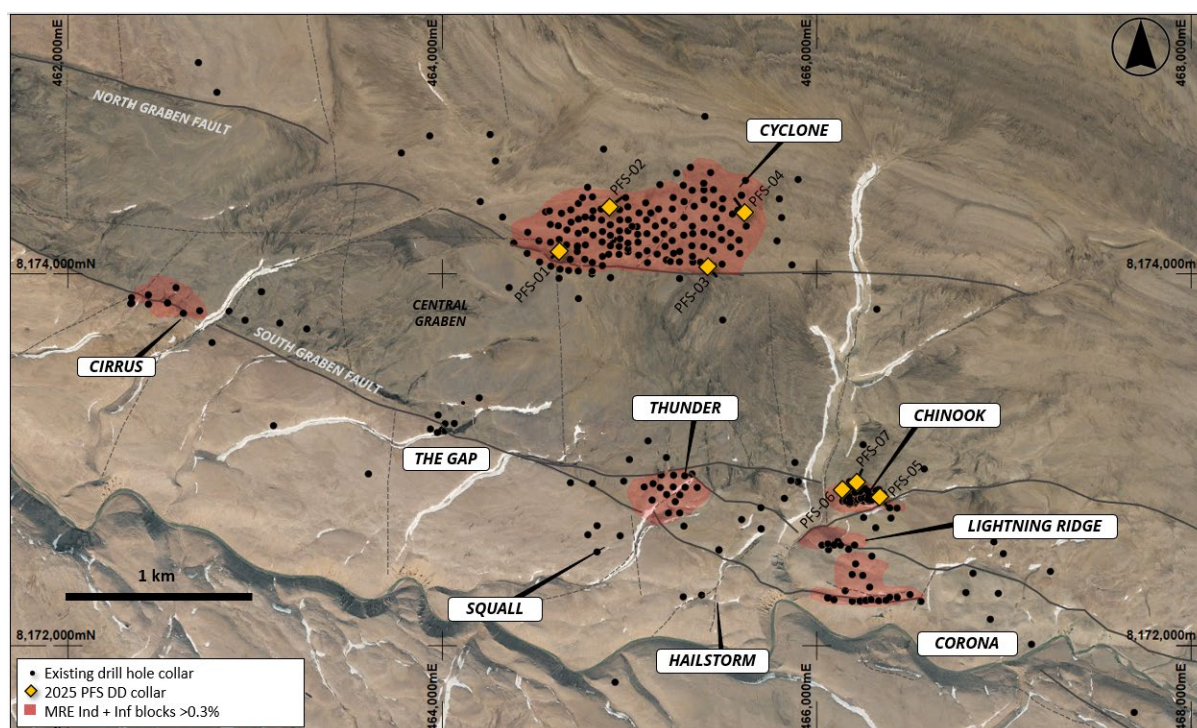
Figure 6: Drill hole locations from the 2025 geotechnical drilling program, overlaying deposit MRE outlines and existing drilling overlaying aerial photography. Section views are located on map.
