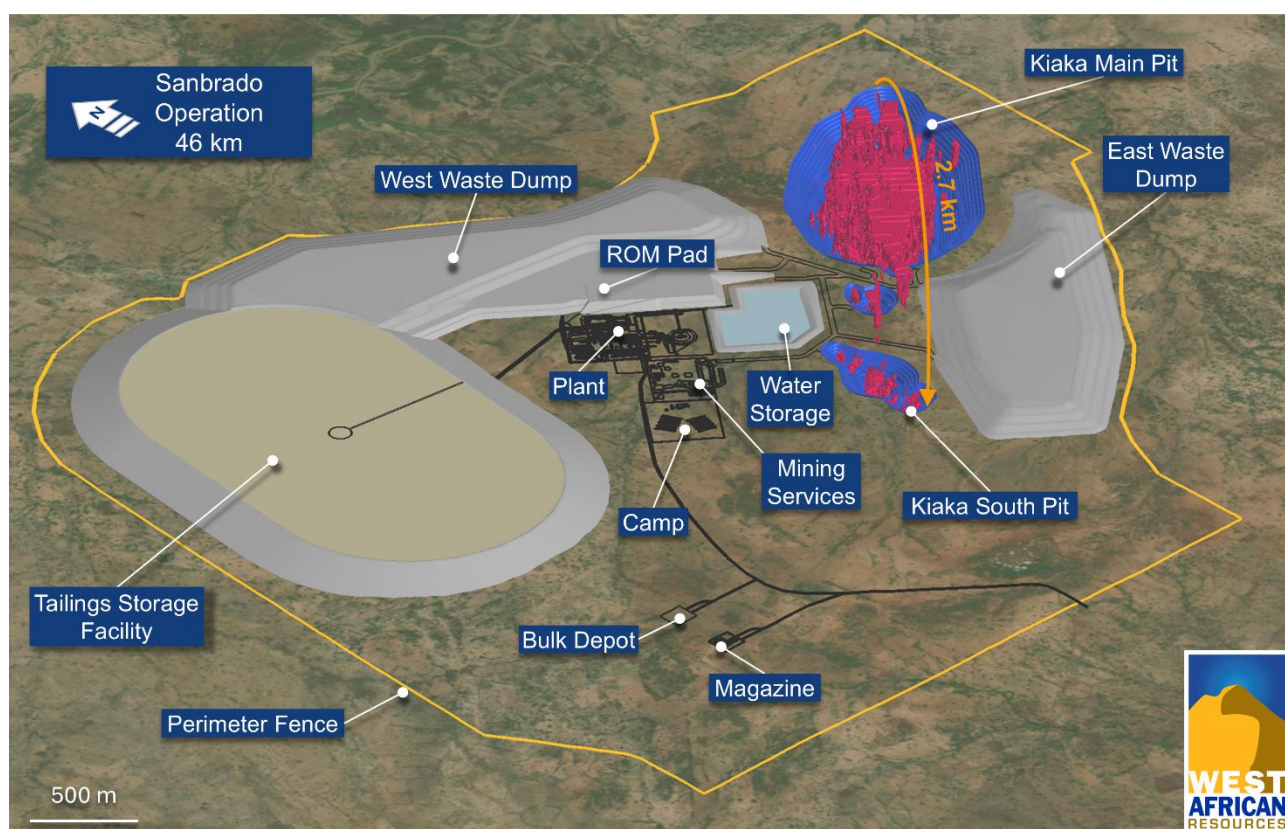
Figure 5 – Kiaka project layout
