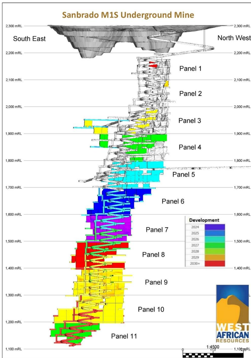
Figure 1 – M1 South underground long section
