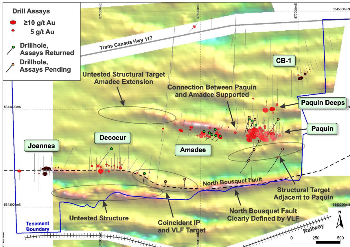
Figure 3: Gold mineralisation in drilling relative to modelled historical VLF EM data
