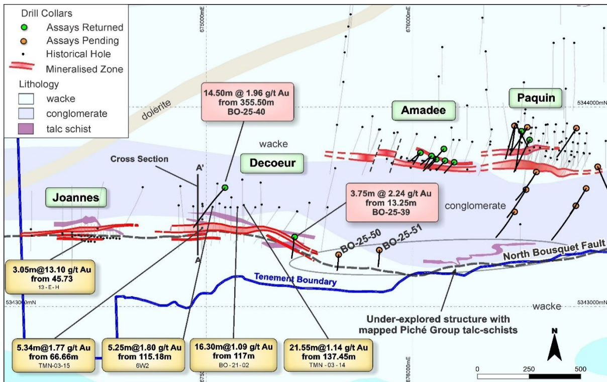
Figure 1: Plan map showing recent drill results for the Decoeur Prospect, Bousquet Gold Project
