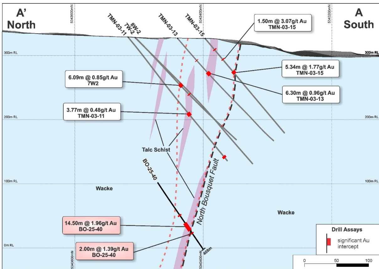
Figure 2: Decoeur cross section A-A' (see Figure 1 for location) showing results for hole BO-25-40. Cross section width 60m.
