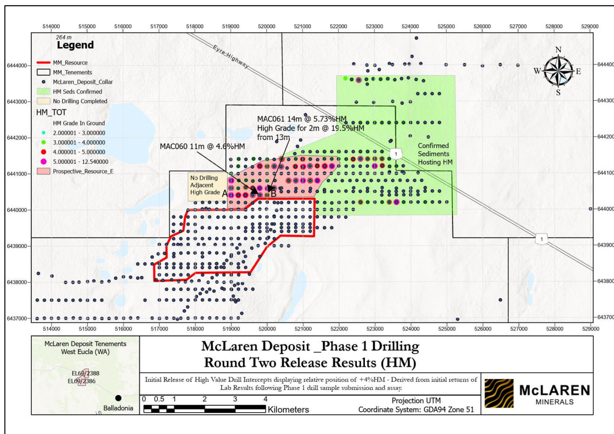
Figure 1: Location of exceptional results noted above, immediately north of existing Indicated Resource Boundary and highlighting the prospective area of resource extension.
