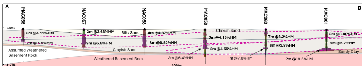
Figure 2: Section showing high-grade results from the area noted on Figure 1 within the Prospective Northern Extension, confirming Mineralisation within previously reported sediments and the identification of a second stacked strand within the geological profile hosting Heavy Minerals.
