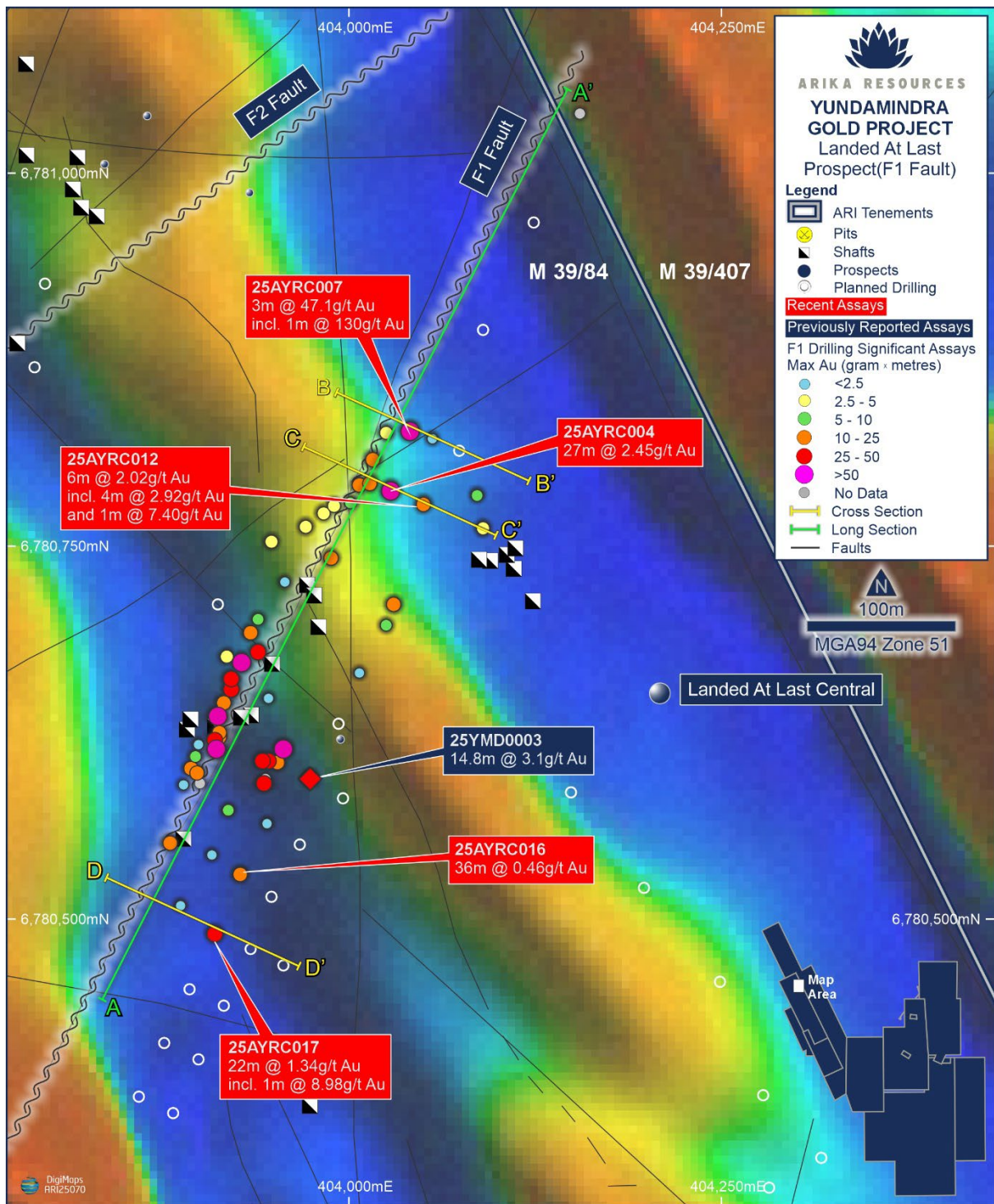
Figure 3: F1 with recent drill collars, significant intercept summaries and proposed holes over TMI.
