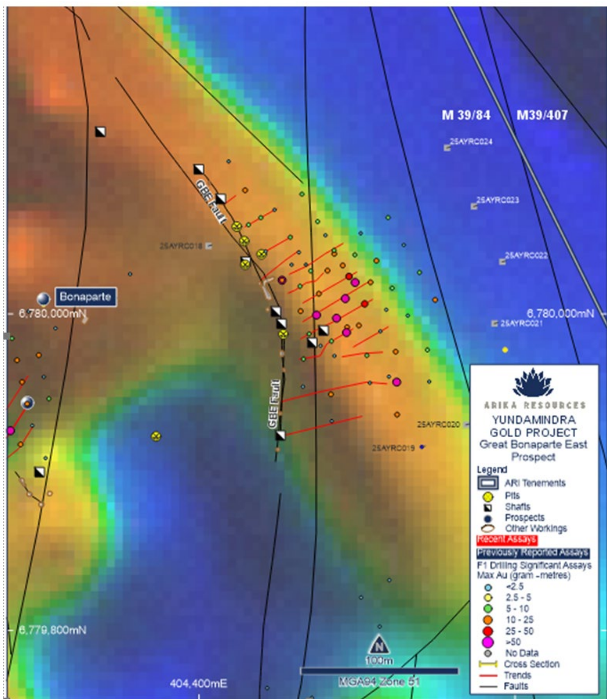
Figure 5: Great Bonaparte East with recent drill collars, significant intercept summaries and proposed holes over TMI.
