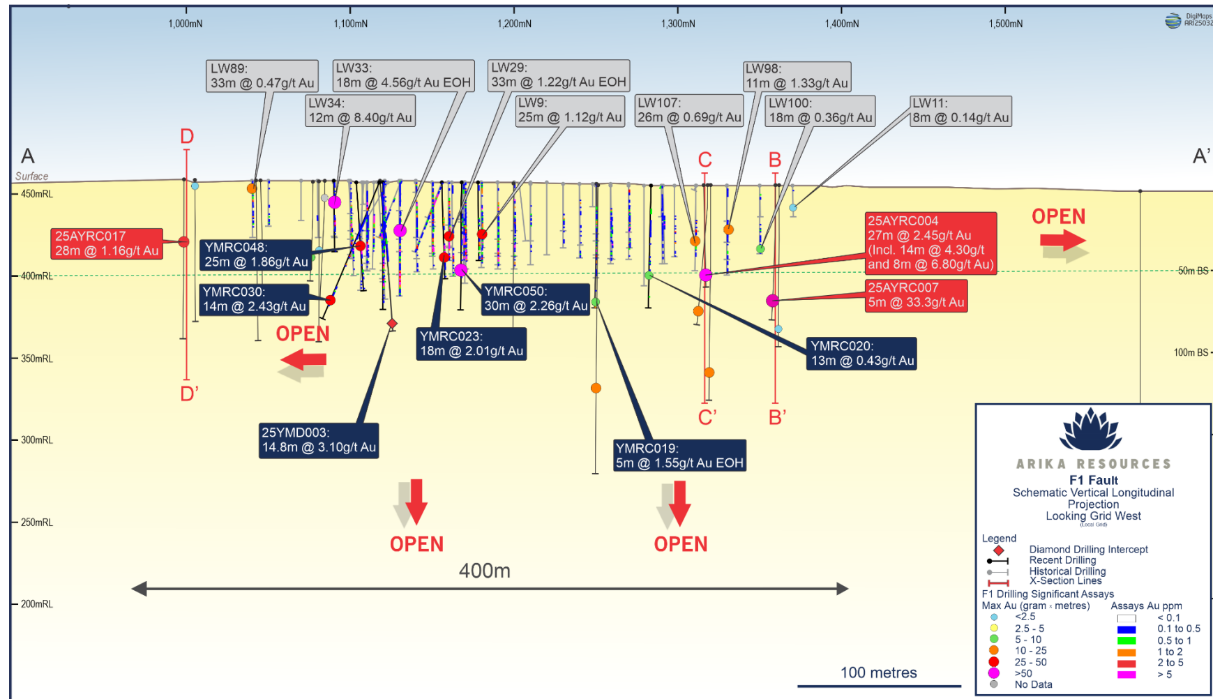
Figure 4: Schematic Vertical Longitudinal Projection (F1-Fault local grid) with recent assay results and historical drilling.
