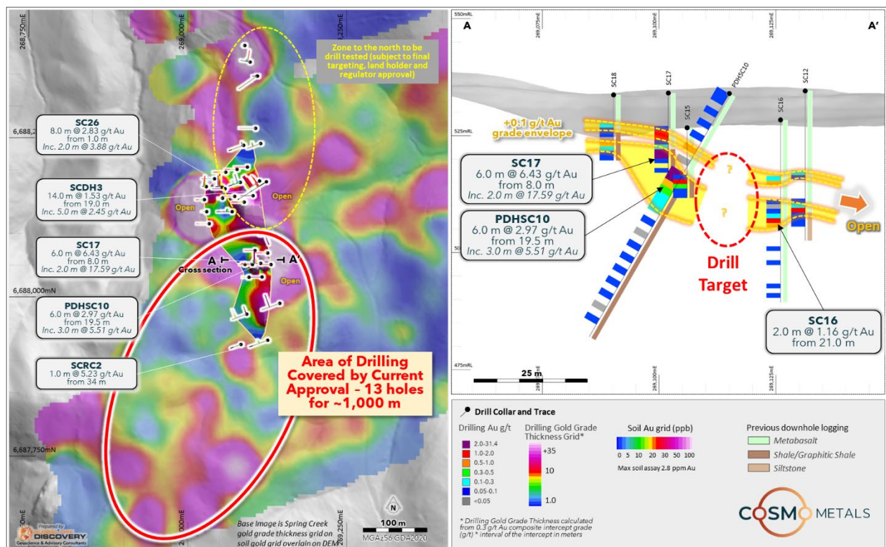
Figure 2. LHS Spring Creek Prospect Drill Intercept Gold Grade * Thickness Grid Showing Area of Planned Drilling; RHS Spring Creek Prospect Cross Section A – A'
