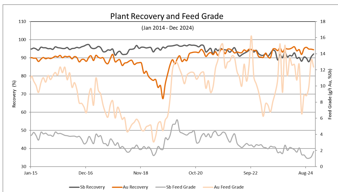
Figure 13.2: Antimony and gold grade versus recovery trends – January 2014 to September 2024
