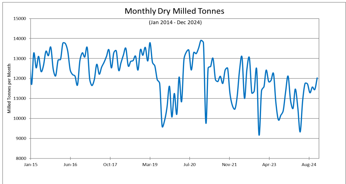
Figure 13.1: Historical Brunswick Processing Plant throughput – 2014 to 2024
