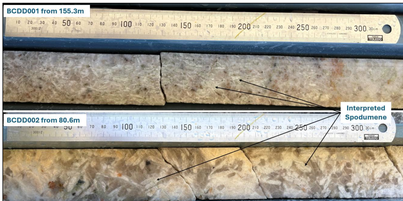
Figure 3: Top : Cut diamond core sample from BCDD001 starting at 155.3m. Abundant slender white elongate crystals are likely spodumene. Bottom : Cut diamond core sample from BCDD002. Large white crystals are likely spodumene. Estimated spodumene abundance is ~40% in both intervals (Table 5).
