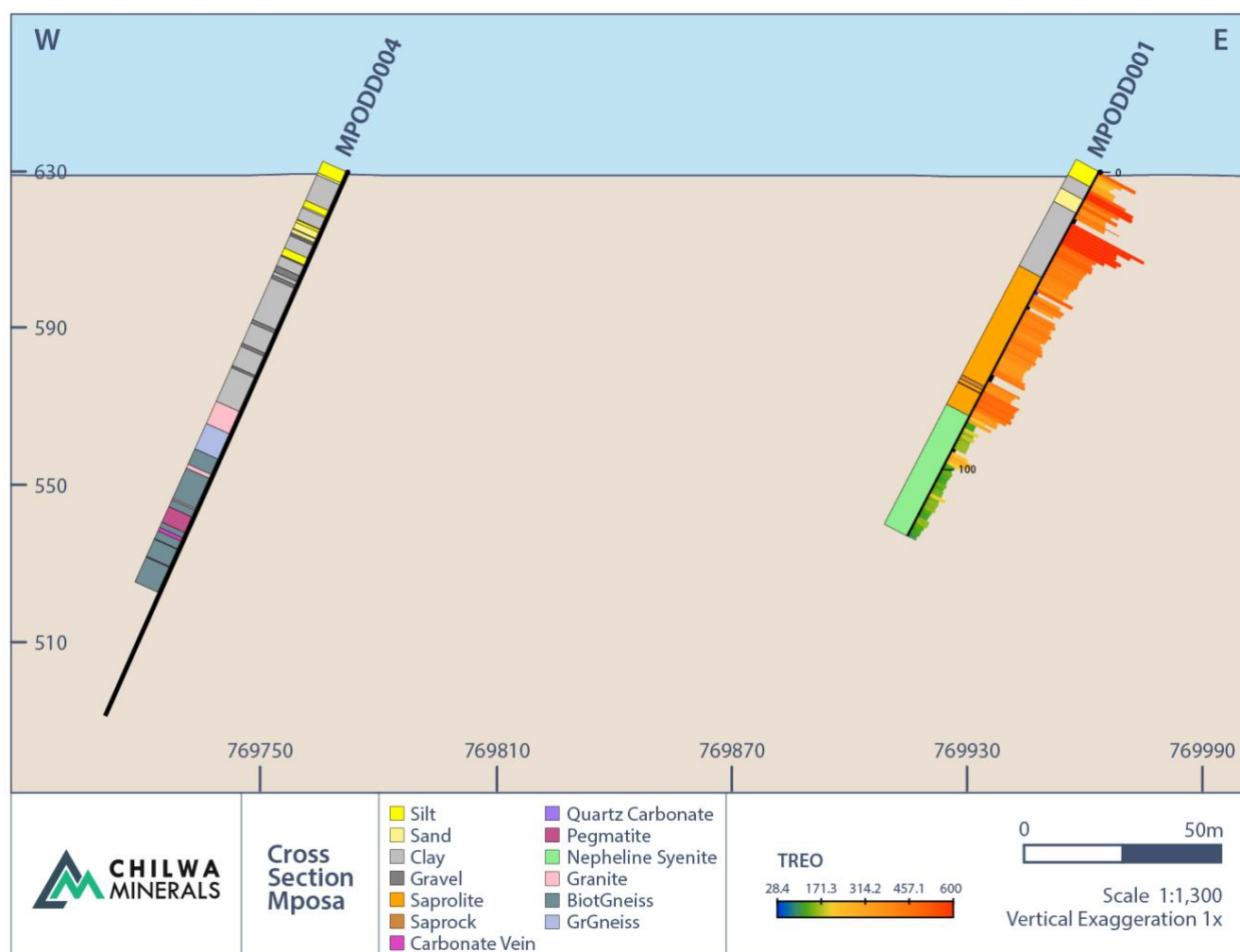
Figure 6: Cross section
