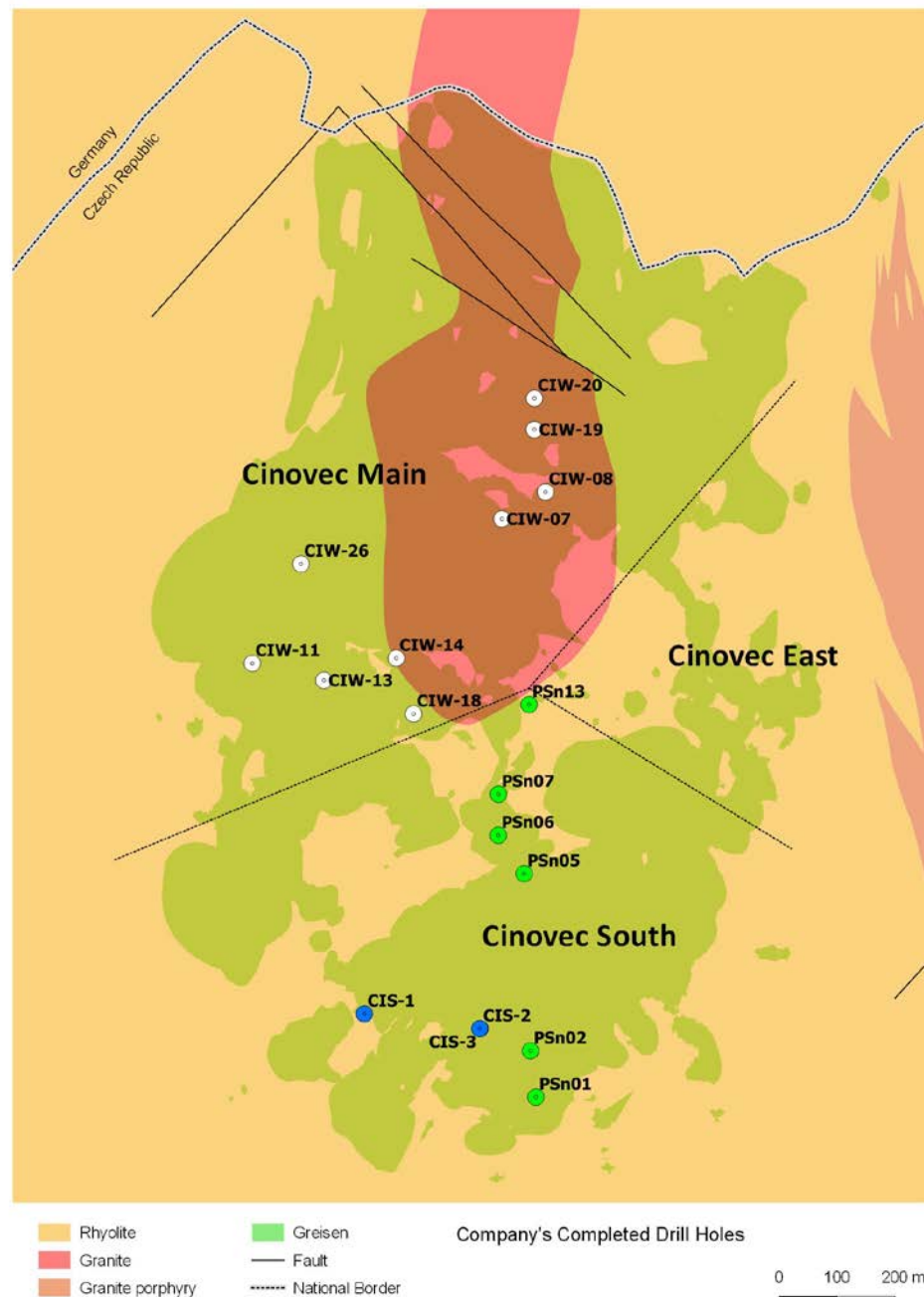
Figure 1 - A geological map showing the Company's drill holes against surface geology and subsurface greisen bodies projected to surface (in green). Historic UG workings and drill holes not shown. Blue and Green circles denote drillholes completed in 2014 and 2015, respectively, 2016 drillholes in white.
