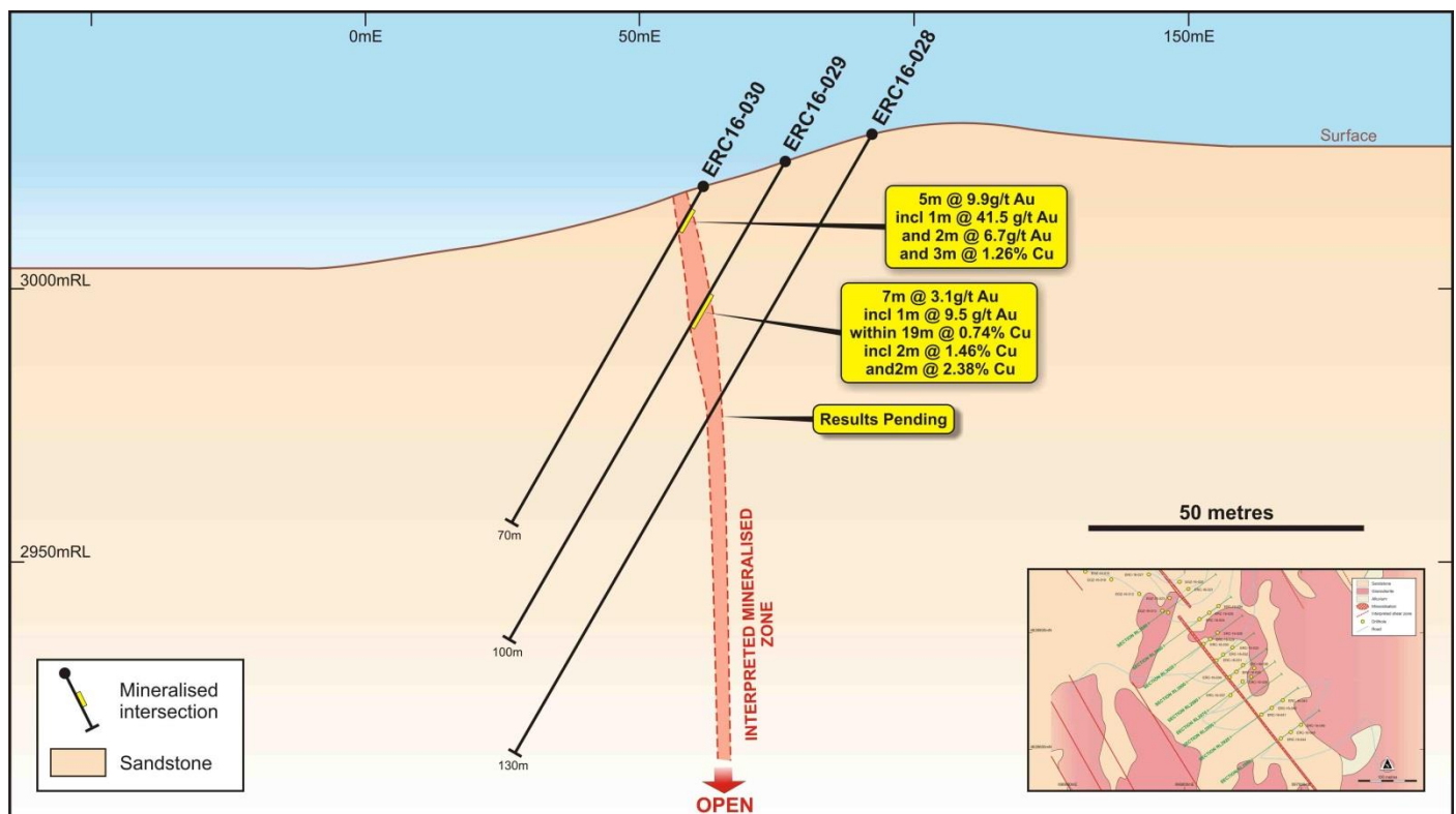
Figure 2: Cross section showing assay results from ERC16-29 and ERC16-30
