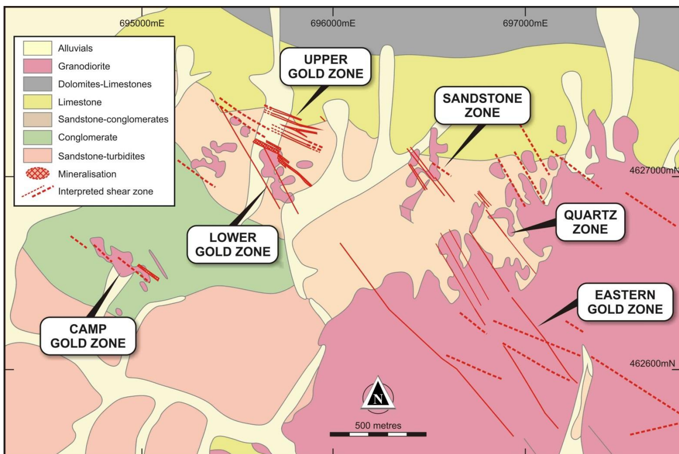
Figure 4: Location map of drilling showing quartz zone and the sandstone zone where visible gold and high grade gold mineralisation is widespread.
