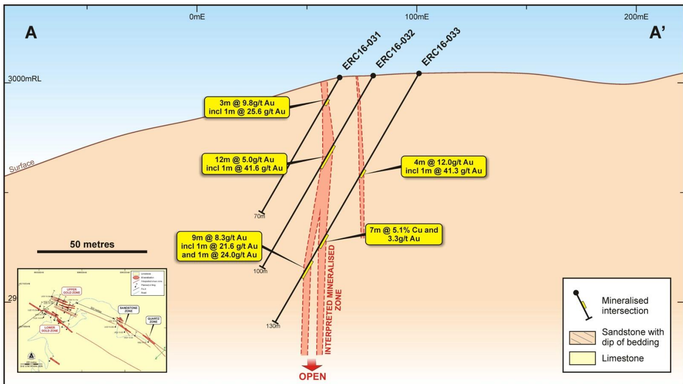
Figure 3: Cross section showing assay results from ERC16-31 to ERC16-33.
