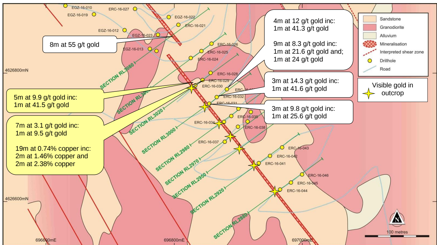
Figure 1: Map showing Quartz Zone and location of outcropping quartz veins (red), drill assay results (new in light yellow text boxes) and completed and planned RC drilling.
